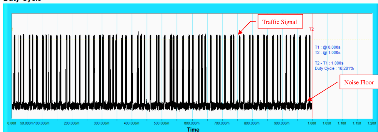
Duty Cycle
