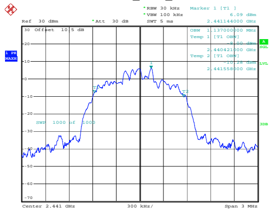
3EDR_DH1_Middle
