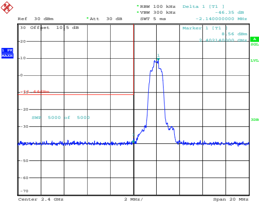
3EDR_DH1_Low
