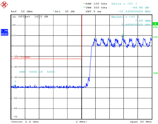
3EDR_DH1_Hopping_Lower
