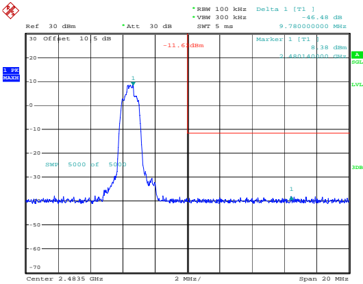
3EDR_DH1_High
