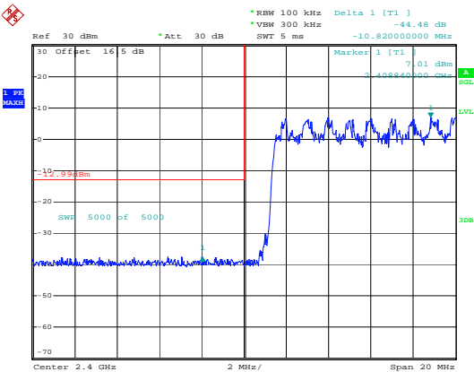
2EDR_DH1_Hopping_Lower
