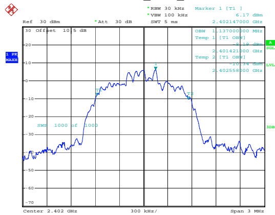
3EDR_DH1_Low
