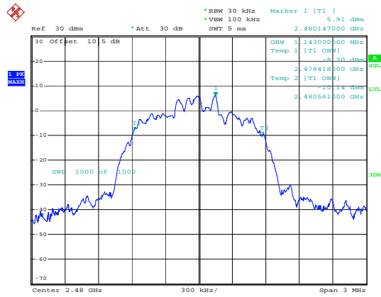
3EDR_DH1_High
