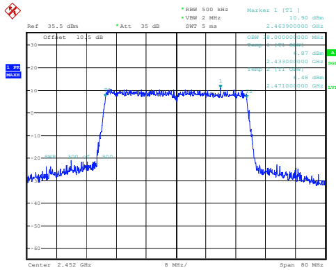
802.11ax40_2452MHz_RU_Full
