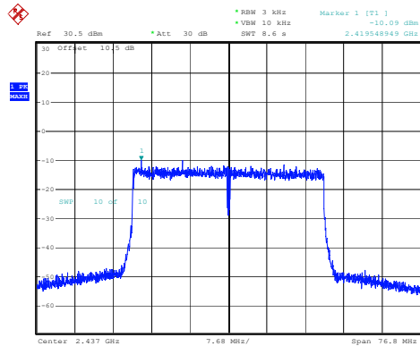
802.11ax40_2437MHz_RU_Full
