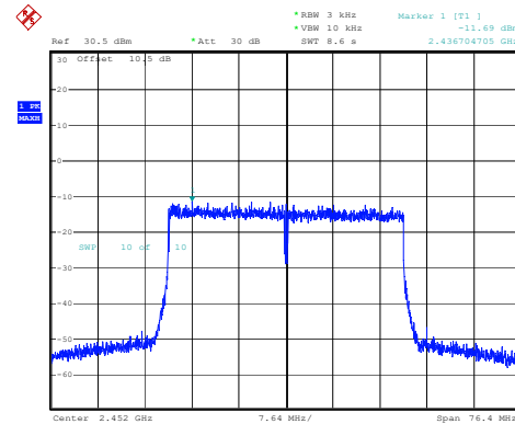
802.11ax40_2452MHz_RU_Full
