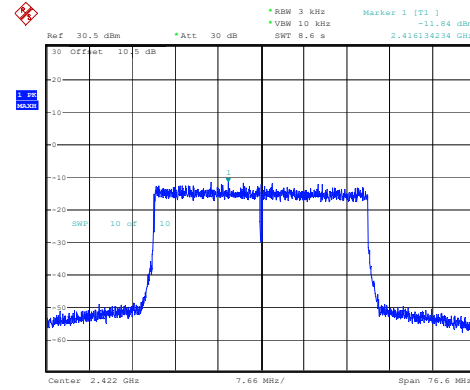
802.11ax40_2422MHz_RU_Full
