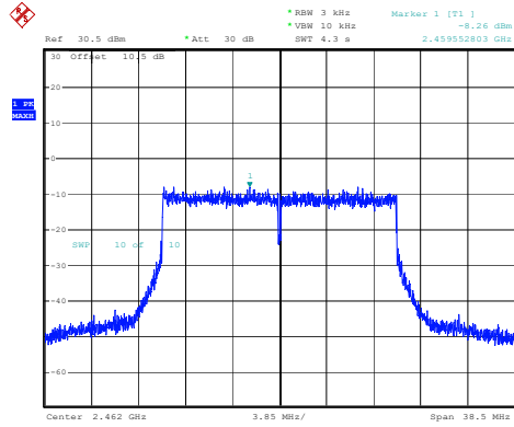
802.11ax20_2462MHz_RU_Full
