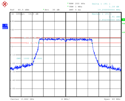
802.11ax20_2462MHz_RU_Full
