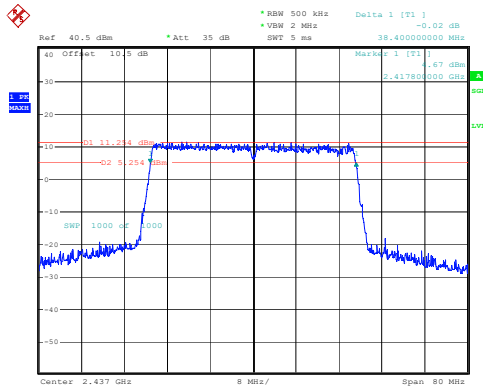
802.11ax40_2437MHz_RU_Full
