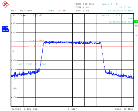
802.11ax40_2422MHz_RU_Full
