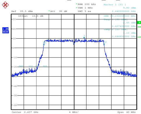
802.11ax20_2437MHz_RU_Full
