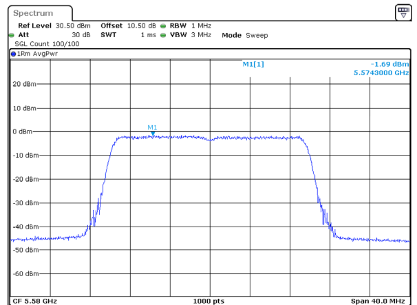
802.11ax20_5580MHz_RU_Full
