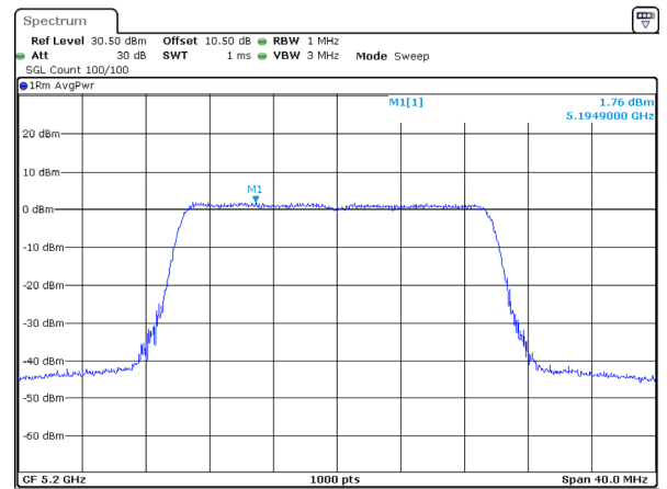
802.11ax20_5200MHz_RU_Full
