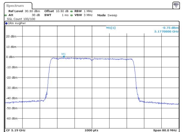
802.11ax40_5190MHz_RU_Full
