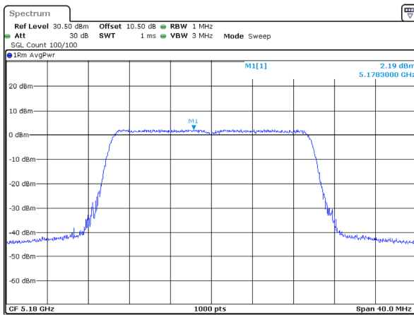
802.11ax20_5180MHz_RU_Full
