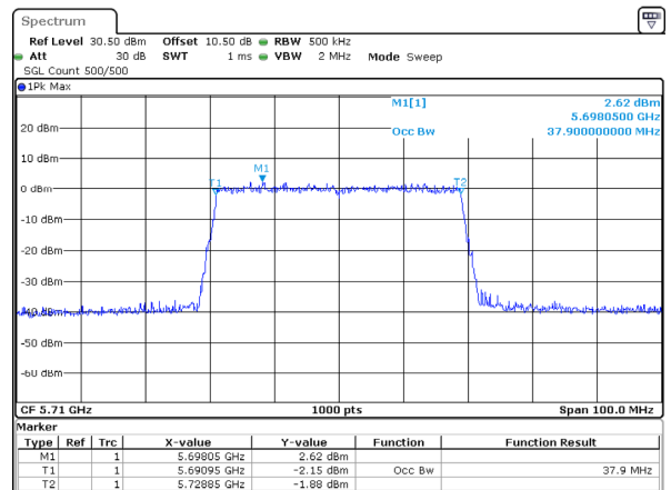
802.11ax40_5710MHz_RU_Full
