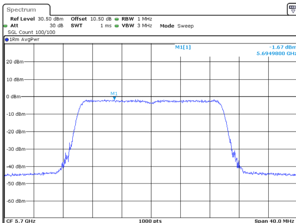
802.11ax20_5700MHz_RU_Full
