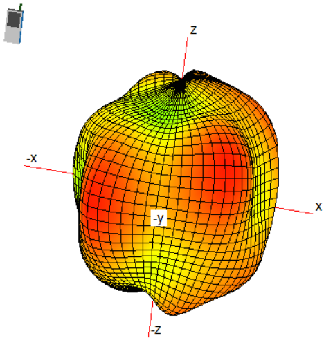
3D Antenna pattern
