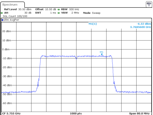
802.11ax40_5755MHz_RU_Full
