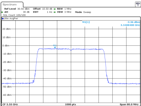
802.11ax40_5550MHz_RU_Full
