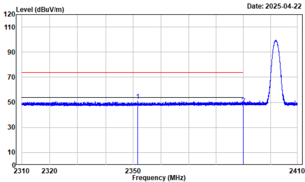
Left Band edge_Horizontal_Peak BT-3DH5-2402MHz
