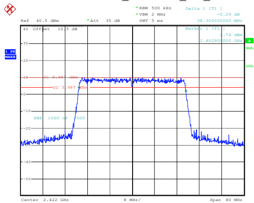
802.11ax40_2422MHz_RU_Full
