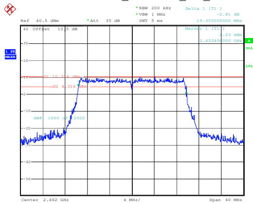
802.11ax20_2462MHz_RU_Full
