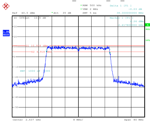
802.11ax40_2437MHz_RU_Full
