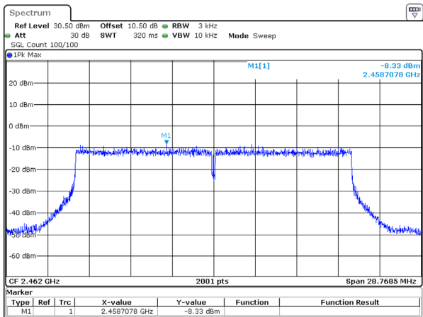
802.11ax20_2462MHz_RU_Full
