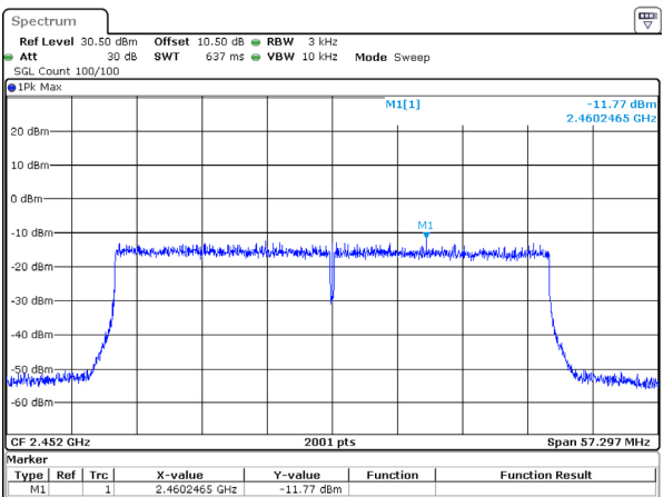
802.11ax40_2452MHz_RU_Full
