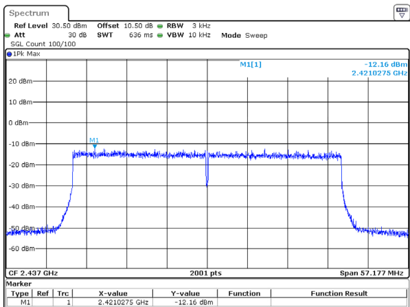
802.11ax40_2437MHz_RU_Full
