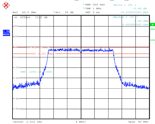
802.11ax20_2412MHz_RU_Full
