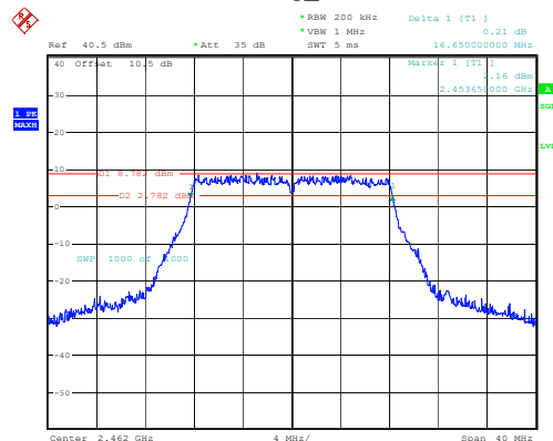
802.11g_2462MHz
