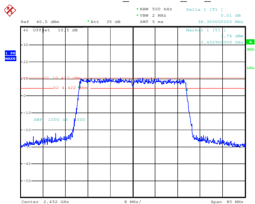
802.11ax40_2452MHz_RU_Full
