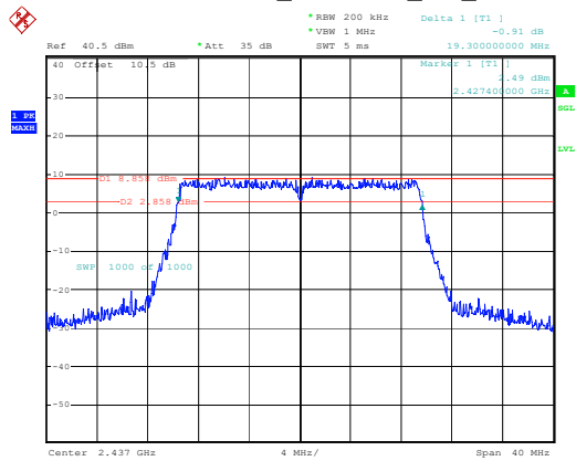
802.11ax20_2437MHz_RU_Full
