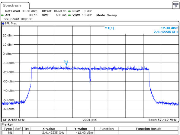
802.11ax40_2422MHz_RU_Full
