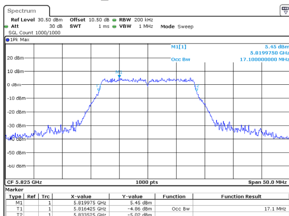
802.11a_5825MHz 17.100MHz
