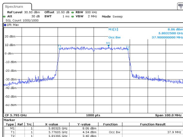
802.11ax40_5795MHz_RU_Full 37.900MHz
