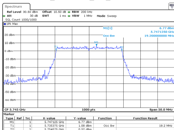
802.11ax20_5745MHz_RU_Full 19.200MHz
