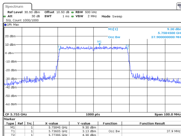
802.11ax40_5755MHz_RU_Full 37.900MHz
