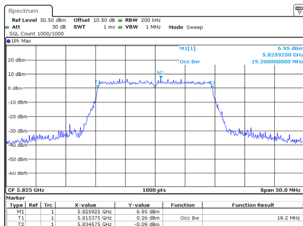
802.11ax20_5825MHz_RU_Full 19.200MHz
