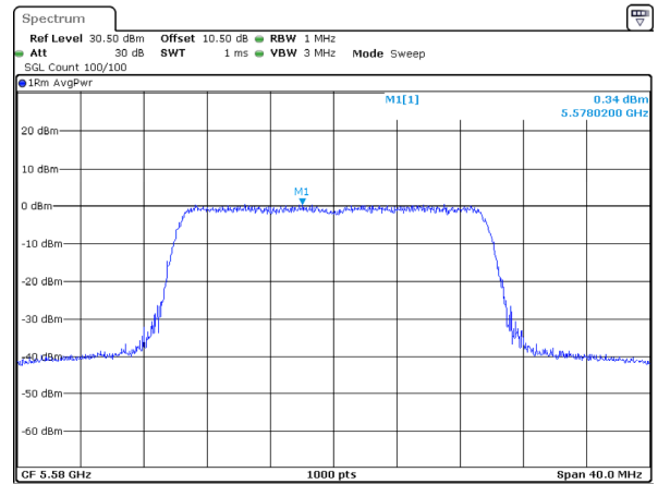
802.11ax20_5580MHz_RU_Full
