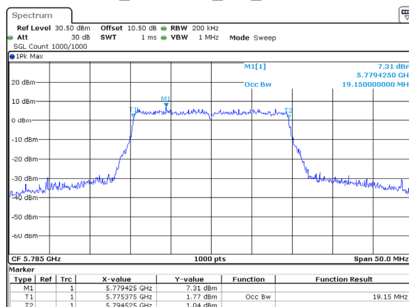
802.11ax20_5785MHz_RU_Full 19.150MHz
