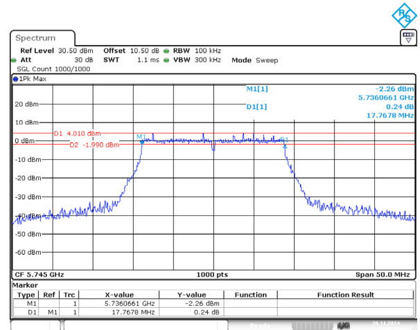
802.11ac20_5745MHz 17.768MHz
