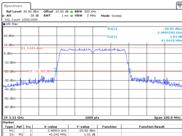
802.11ac40_5510MHz 41.041MHz
