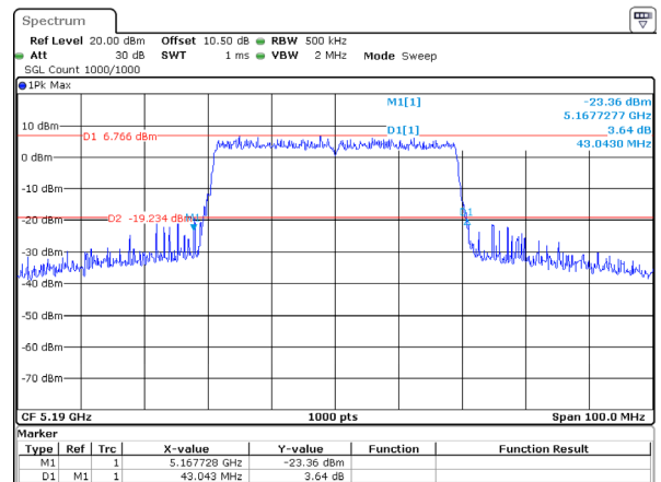
802.11ax40_5190MHz_RU_Full 43.043MHz
