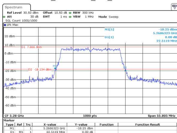
802.11ax20_5280MHz_RU_Full 22.512MHz
