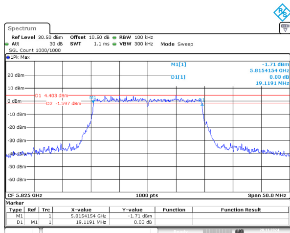
802.11ax20_5825MHz_RU_Full 19.119MHz
