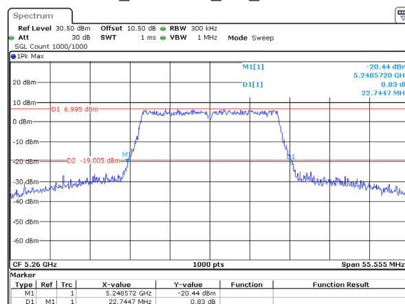
802.11ax20_5260MHz_RU_Full 22.745MHz
