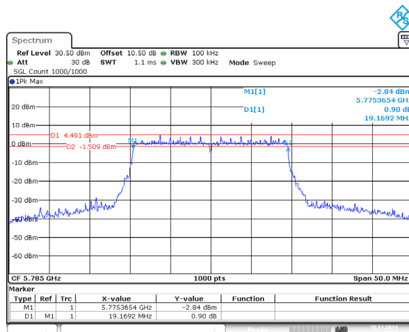
802.11ax20_5785MHz_RU_Full 19.169MHz
