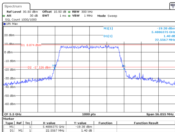
802.11ax20_5500MHz_RU_Full 22.557MHz
