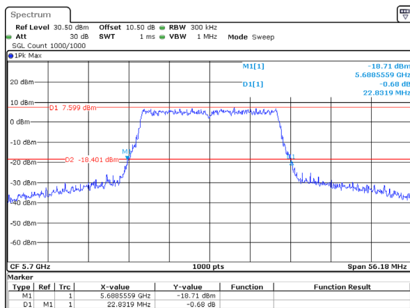
802.11ax20_5700MHz_RU_Full 22.832MHz
