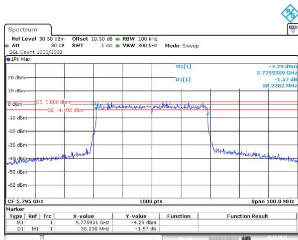
802.11ax40_5795MHz_RU_Full 38.238MHz
