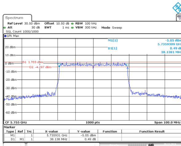
802.11ax40_5755MHz_RU_Full 38.138MHz
