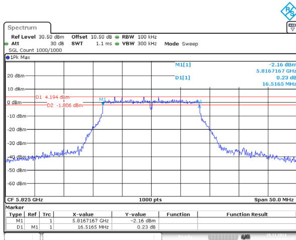
802.11a_5825MHz 16.517MHz
