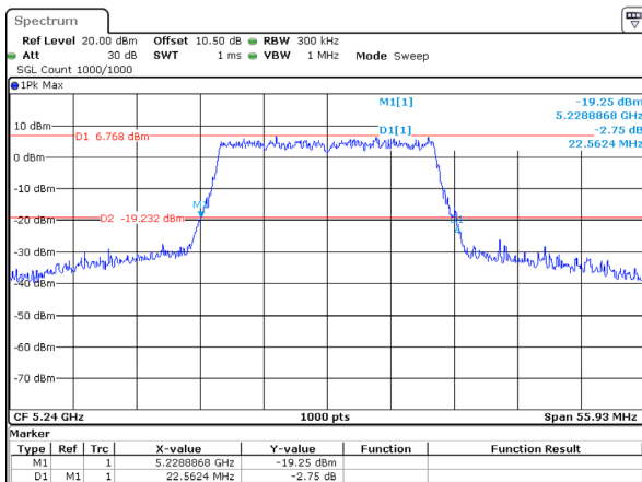
802.11ax20_5240MHz_RU_Full 22.562MHz
