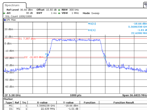
802.11ax20_5580MHz_RU_Full 22.639MHz
