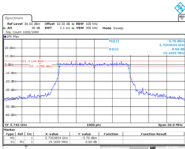
802.11ax20_5745MHz_RU_Full 19.169MHz
