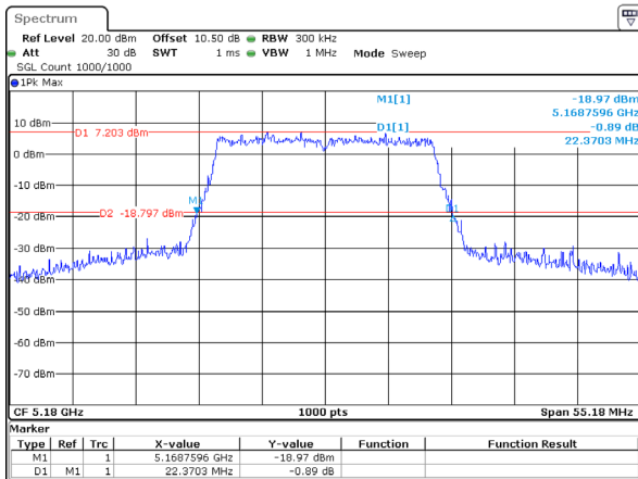
802.11ax20_5180MHz_RU_Full 22.370MHz
