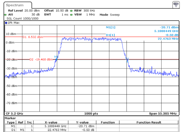
802.11ax20_5200MHz_RU_Full 22.476MHz
