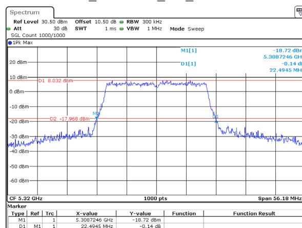
802.11ax20_5320MHz_RU_Full 22.494MHz
