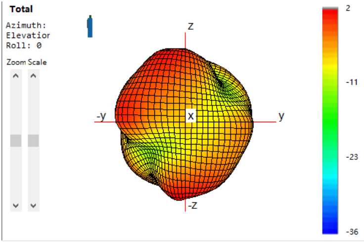
3D Antenna pattern
