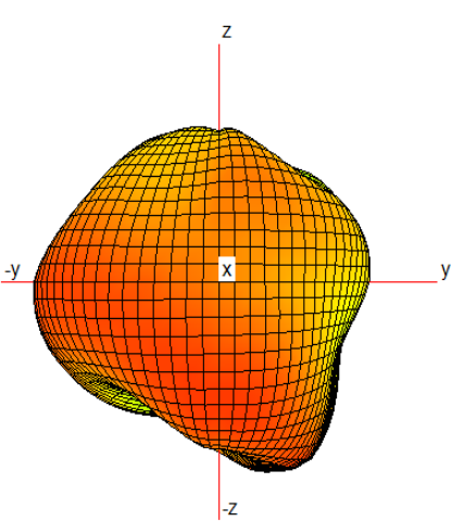
3D Antenna pattern
