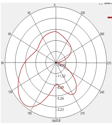
2D Antenna pattern (X->Y;X->Z;Y->Z)
