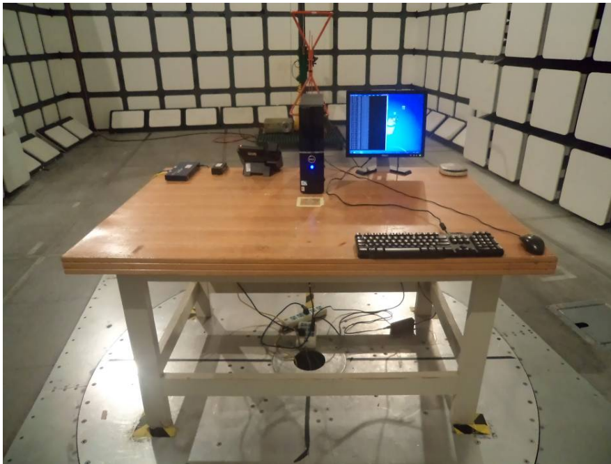
Below 1 GHz: Radiated Emissions - Front View (PoE power supply)
