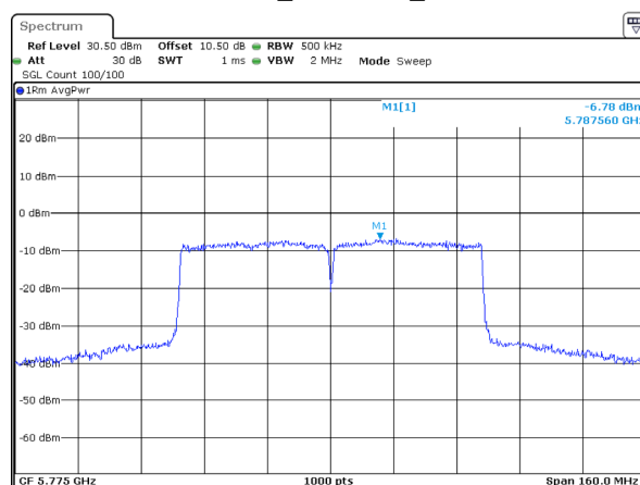
802.11ac80_5775MHz_Chain 1
