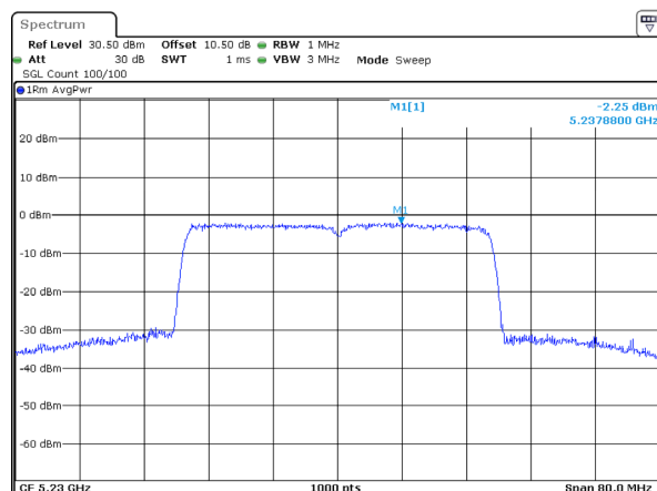
802.11ax40_5230MHz_RU_Full_Chain 0
