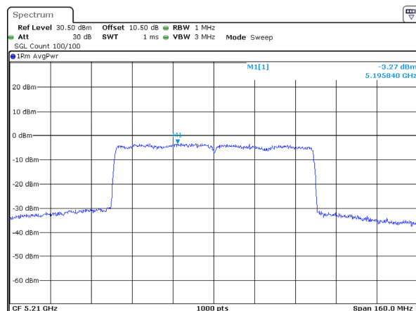
802.11ax80_5210MHz_RU_Full_Chain 1
