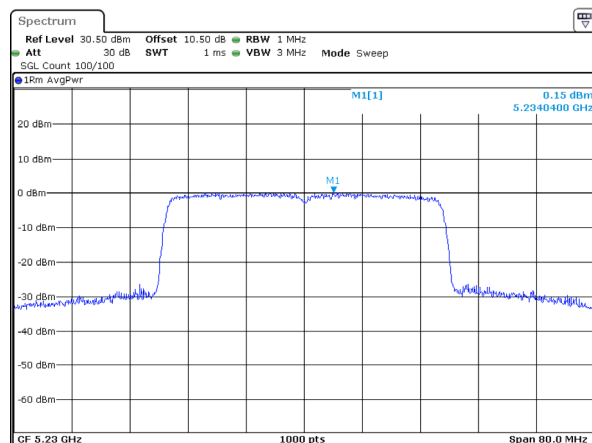
802.11ax40_5230MHz_RU_Full_Chain 1
