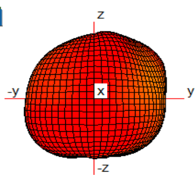
3D Antenna pattern
