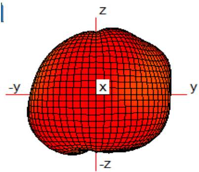
3D Antenna pattern
