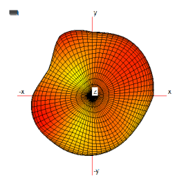
2484MHz 3D Antenna Graph
