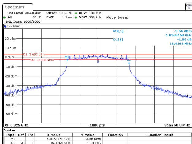
802.11a_5825MHz
