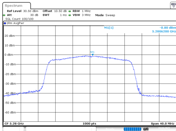
802.11ax20_5280MHz_RU_Full_Chain 1
