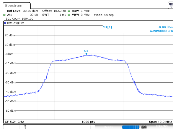
802.11n20_5240MHz_Chain 0
