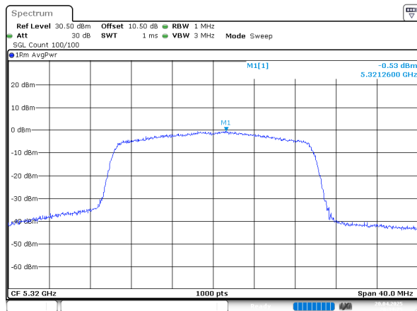
802.11ax20_5320MHz_RU_Full_Chain 0
