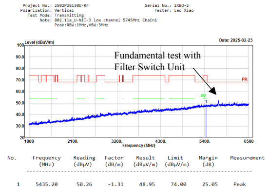
802.11a, Low Channel, Vertical
