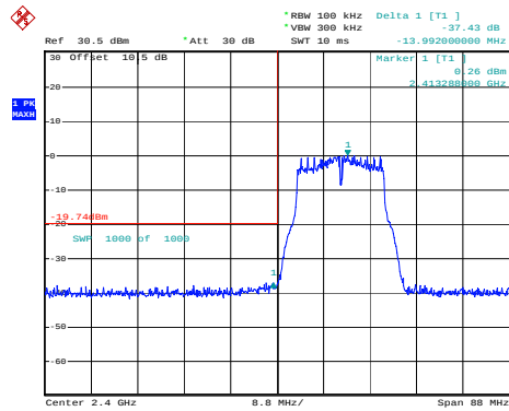
802.11g_2412MHz_Chain 1
