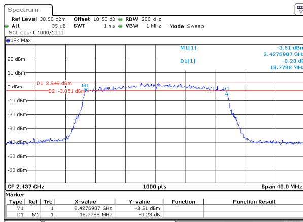
802.11ax20_2437MHz_RU_Full_Chain 1
