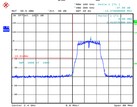
802.11g_2412MHz_Chain 0
