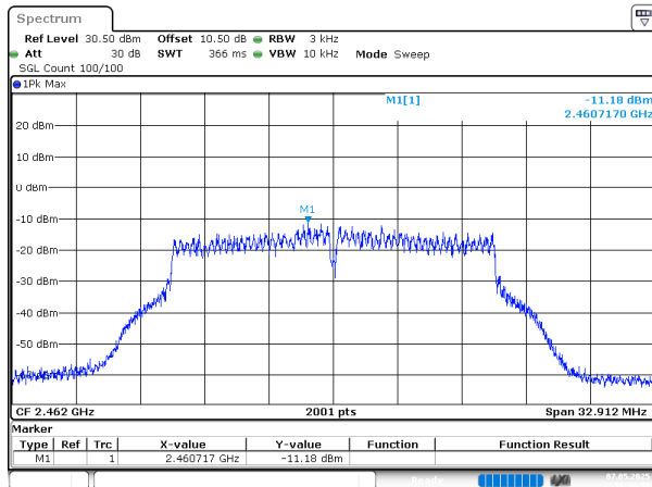
802.11g_2462MHz_Chain 0
