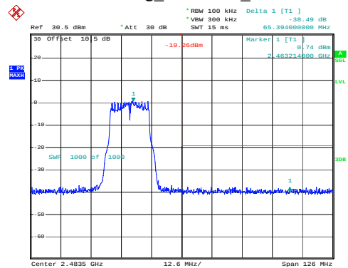
802.11g_2462MHz_Chain 0
