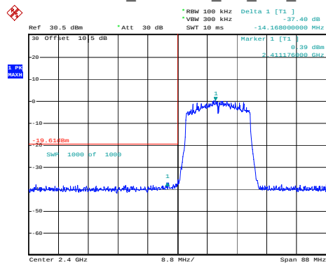
802.11ax20_2412MHz_RU_Full_Chain 0
