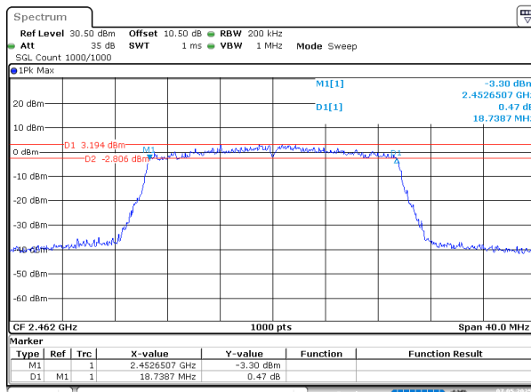
802.11ax20_2462MHz_RU_Full_Chain 0
