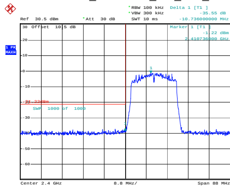
802.11ax20_2412MHz_RU_Full_Chain 1
