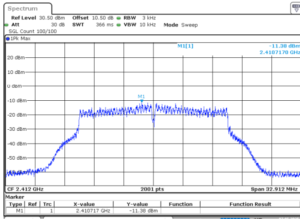
802.11g_2412MHz_Chain 0
