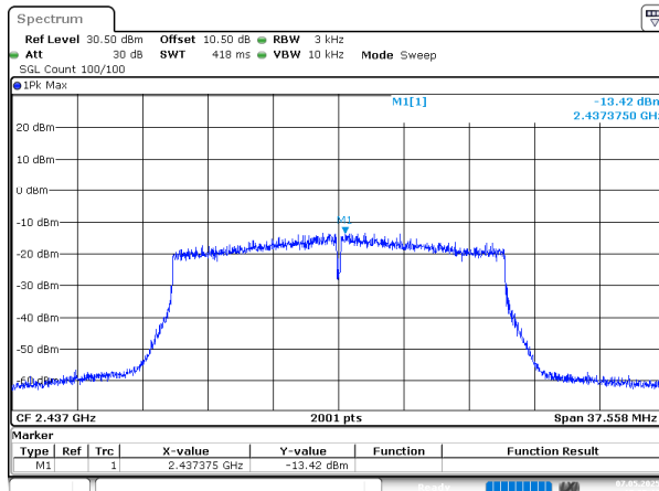
802.11ax20_2437MHz_RU_Full_Chain 1
