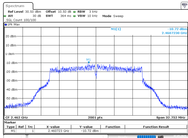
802.11g_2462MHz_Chain 1
