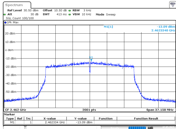
802.11ax20_2462MHz_RU_Full_Chain 1
