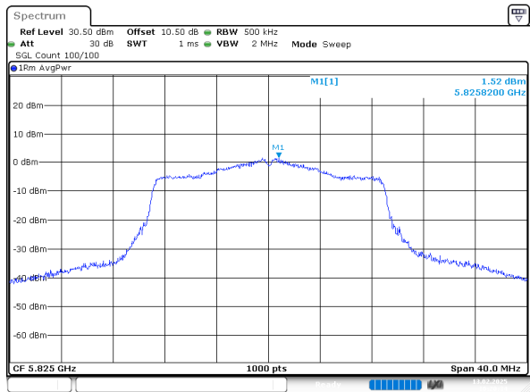
802.11n20_5825MHz_Chain 0
