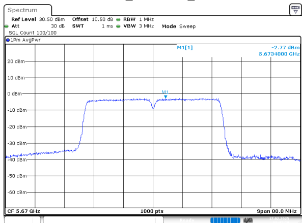
802.11n40_5670MHz_Chain 1
