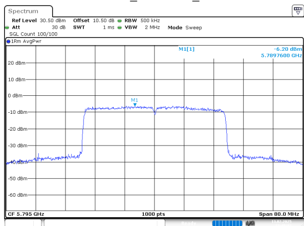
802.11ax40_5795MHz_Chain 0
