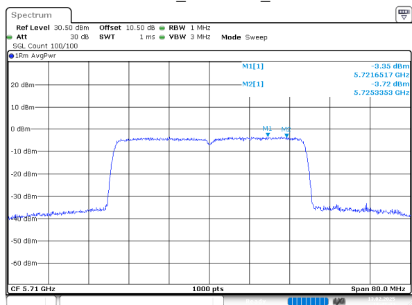
802.11ax40_5710MHz_Chain 0
