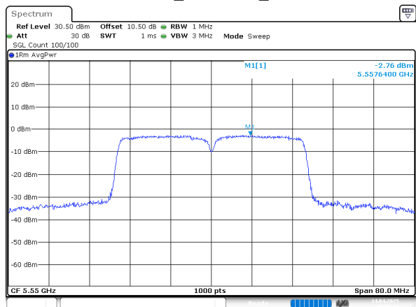
802.11n40_5550MHz_Chain 0
