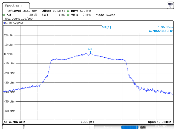
802.11n20_5785MHz_Chain 1
