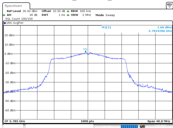
802.11n20_5785MHz_Chain 0
