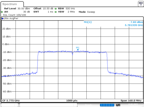
802.11ax80_5775MHz_Chain 0
