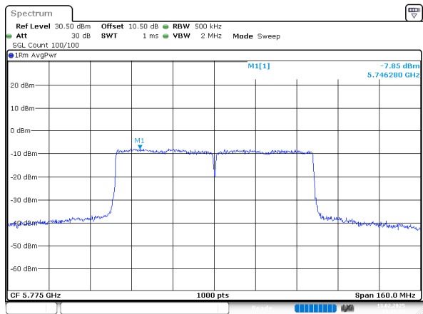
802.11ac80_5775MHz_Chain 0
