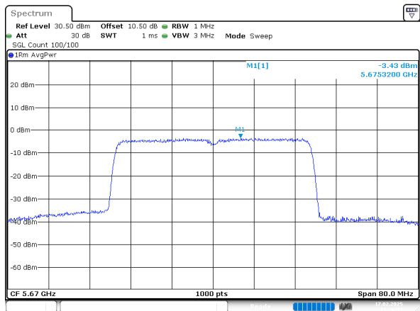
802.11ax40_5670MHz_Chain 1
