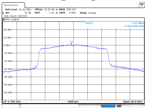
802.11ax20_5785MHz_Chain 1
