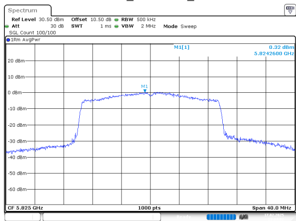
802.11ax20_5825MHz_Chain 1
