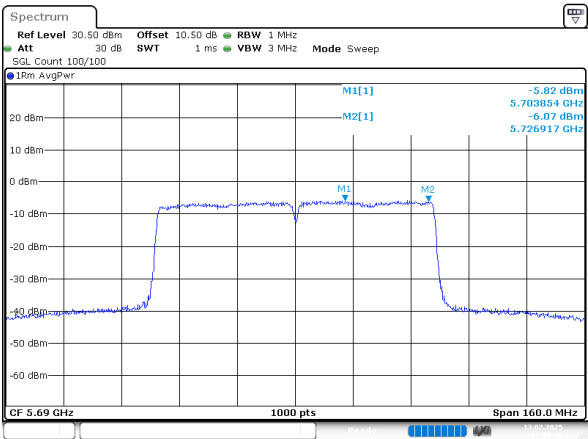
802.11ac80_5690MHz_Chain 0
