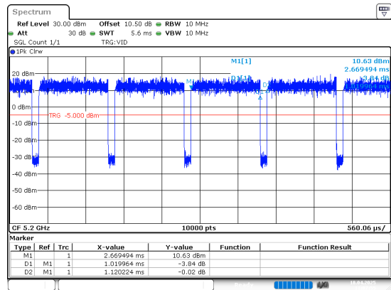
802.11ax20_5200MHz_Chain 0
