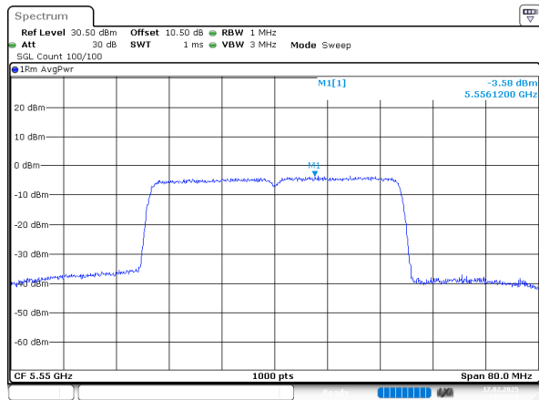
802.11ax40_5550MHz_Chain 1
