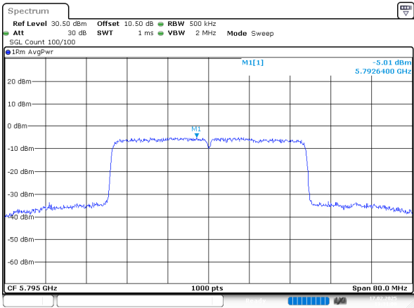
802.11ax40_5795MHz_Chain 1
