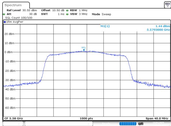
802.11ax20_5580MHz_Chain 0
