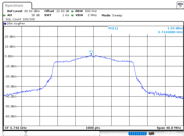
802.11n20_5745MHz_Chain 1
