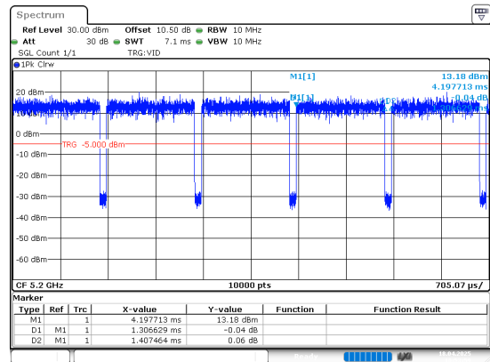
802.11n20_5200MHz_Chain 0
