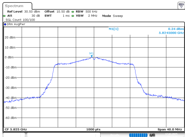
802.11n20_5825MHz_Chain 1
