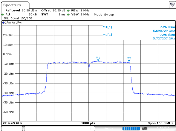
802.11ac80_5690MHz_Chain 1
