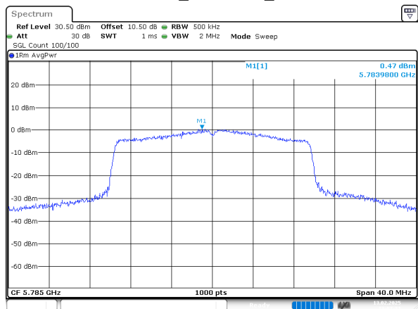
802.11ax20_5785MHz_Chain 0
