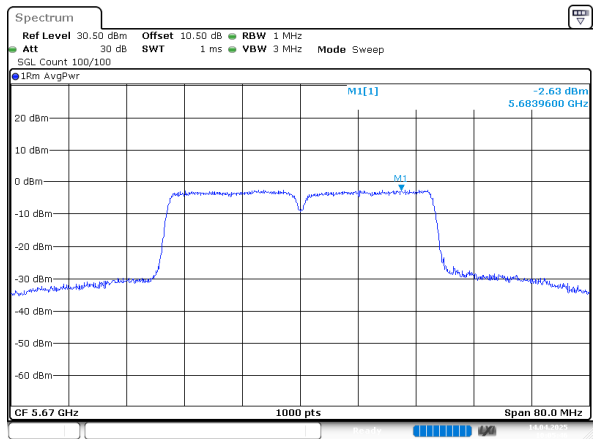
802.11n40_5670MHz_Chain 0
