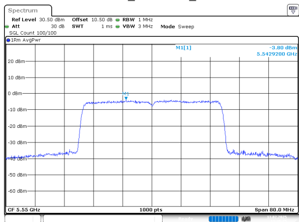
802.11ax40_5550MHz_Chain 0
