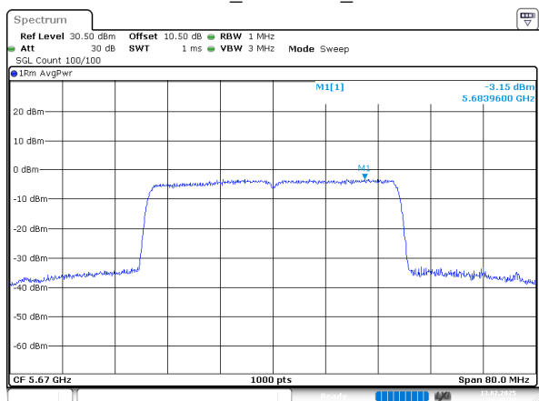
802.11ax40_5670MHz_Chain 0
