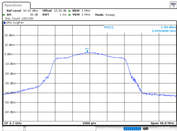
802.11a_5700MHz_Chain 1
