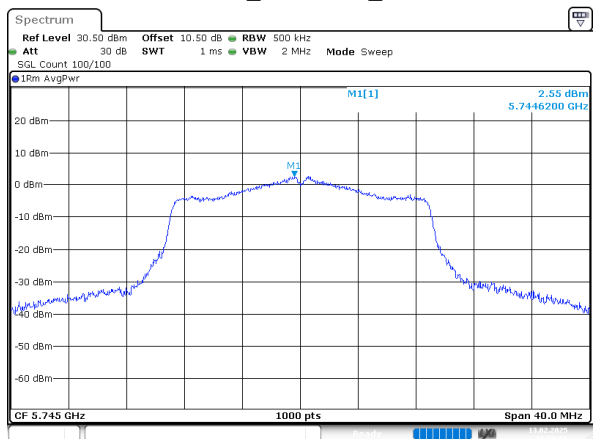
802.11n20_5745MHz_Chain 0
