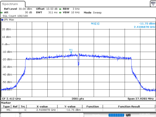
802.11ax20_2412MHz_Chain 0
