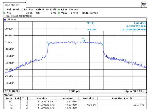
802.11ax20_5180MHz_RU_Full
