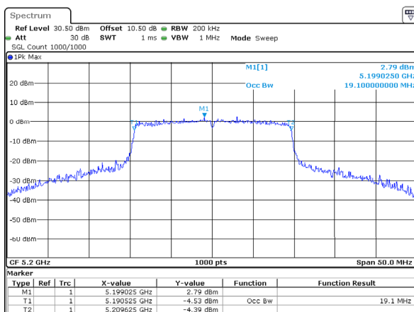
802.11ax20_5200MHz_RU_Full
