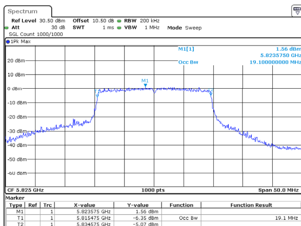
802.11ax20_5825MHz_RU_Full
