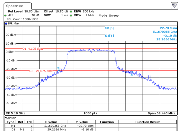
802.11ax20_5180MHz_RU_Full
