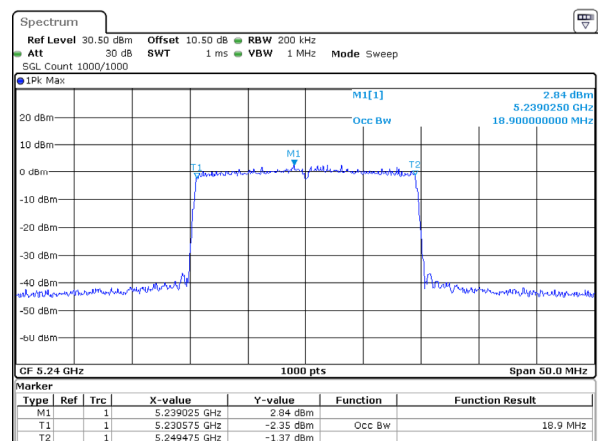
802.11ax20_5240MHz_RU_Full
