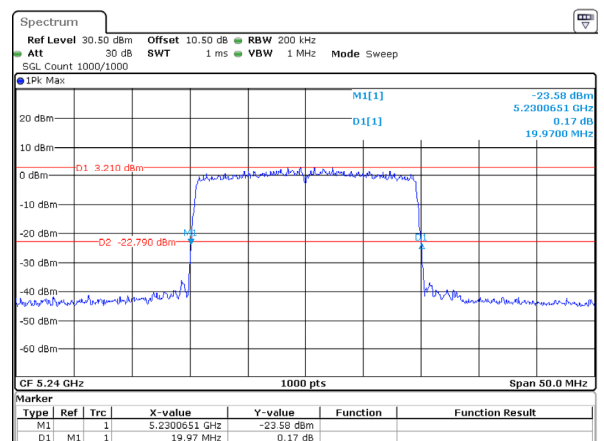
802.11ax20_5240MHz_RU_Full
