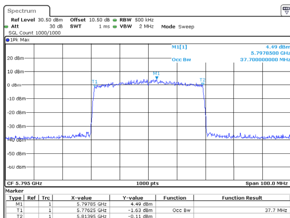
802.11ax40_5795MHz_RU_Full
