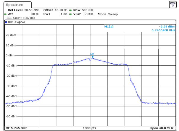
802.11ac20_5745MHz_Chain 2
