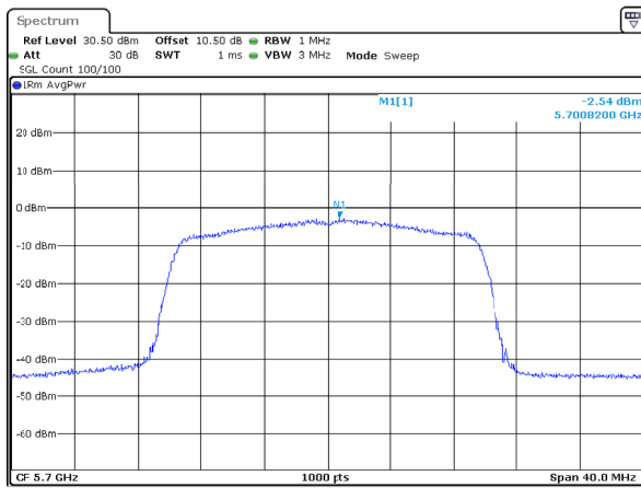
802.11ax20_5700MHz_RU_Full_Chain 2
