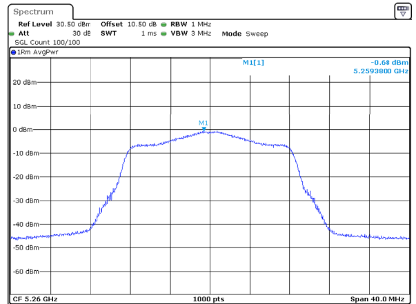
802.11a_5260MHz_Chain 2
