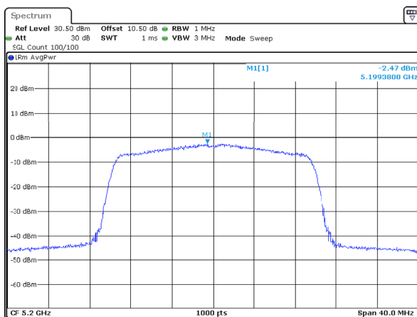
802.11ax20_5200MHz_RU_Full_Chain 2
