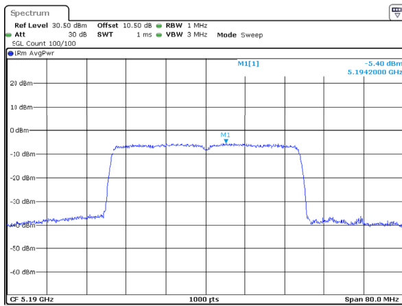
802.11ax40_5190MHz_RU_Full_Chain 1
