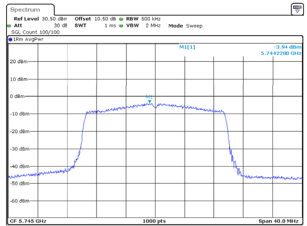
802.11ax20_5745MHz_RU_Full_Chain 2
