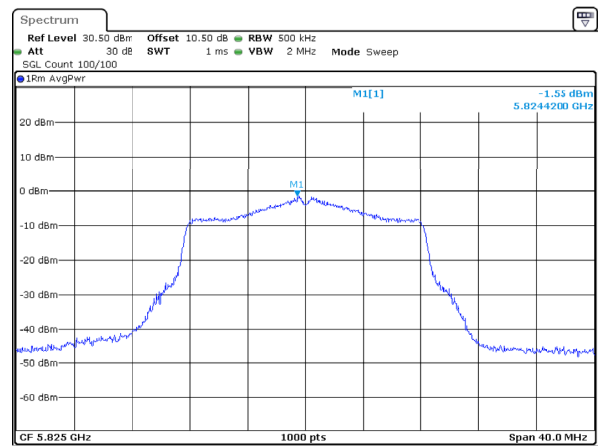
802.11a_5825MHz_Chain 2
