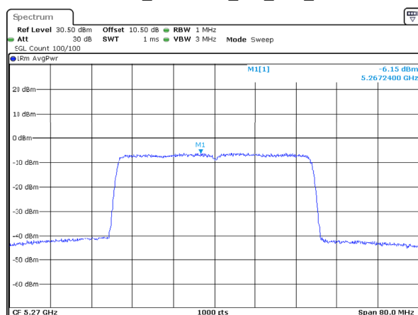
802.11ax40_5270MHz_RU_Full_Chain 2
