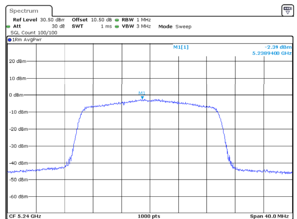
802.11ax20_5240MHz_RU_Full_Chain 2
