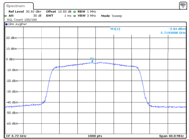
802.11ax20_5720MHz_RU_Full_Chain 2
