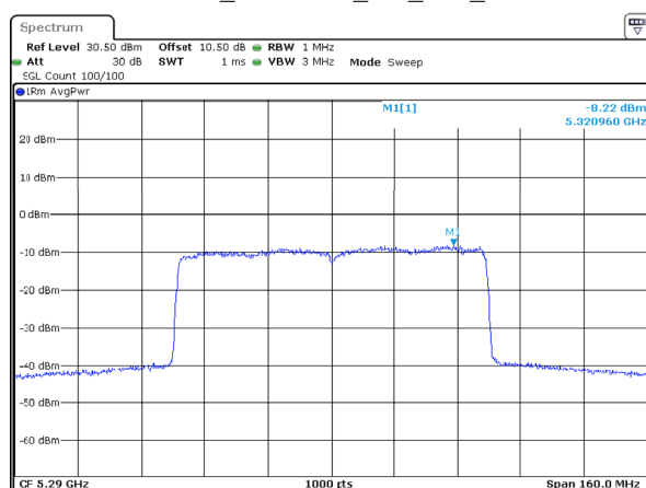
802.11ax80_5290MHz_RU_Full_Chain 1
