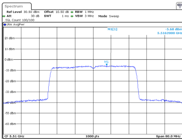
802.11ax40_5510MHz_RU_Full_Chain 1
