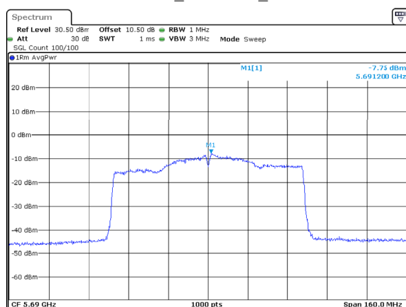
802.11ac80_5690MHz_Chain 2
