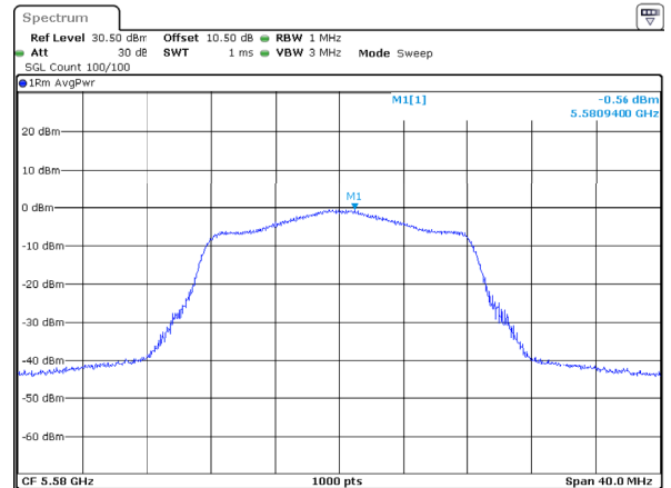
802.11a_5580MHz_Chain 1
