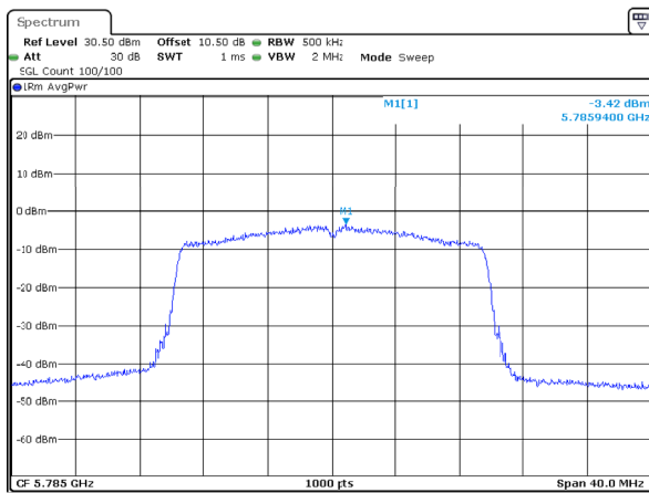
802.11ax20_5785MHz_RU_Full_Chain 2
