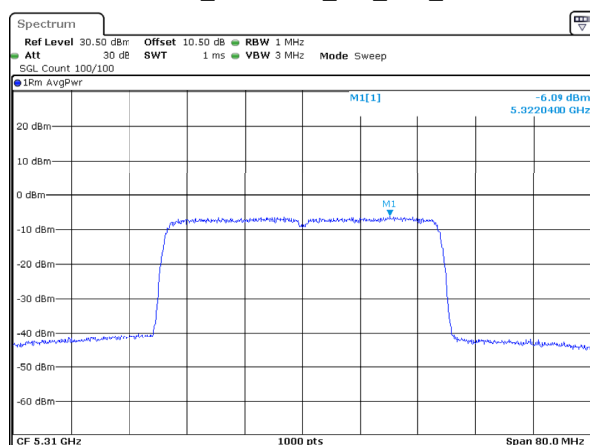
802.11ax40_5310MHz_RU_Full_Chain 2
