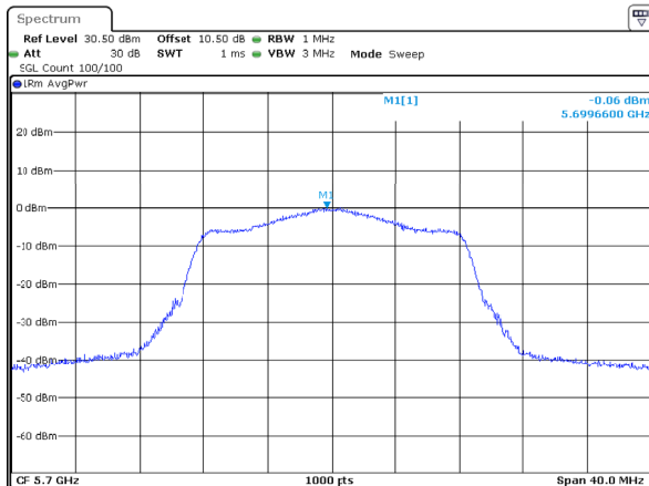
802.11a_5700MHz_Chain 1
