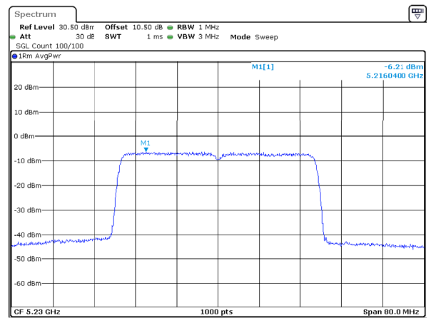
802.11ax40_5230MHz_RU_Full_Chain 2
