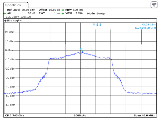
802.11a_5745MHz_Chain 2
