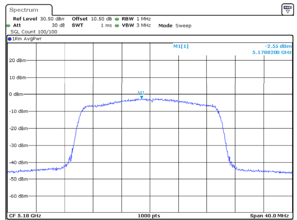
802.11ax20_5180MHz_RU_Full_Chain 2
