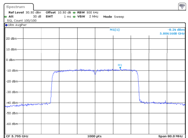
802.11ax40_5795MHz_RU_Full_Chain 1
