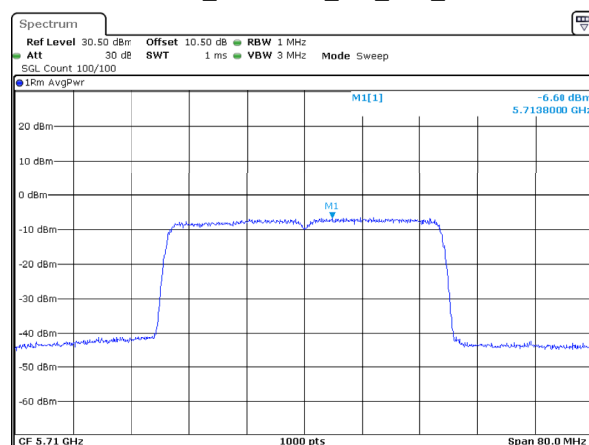
802.11ax40_5710MHz_RU_Full_Chain 2
