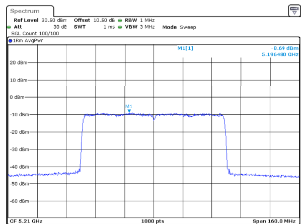
802.11ax80_5210MHz_RU_Full_Chain 2
