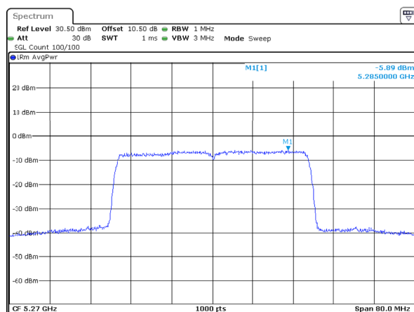
802.11ax40_5270MHz_RU_Full_Chain 1
