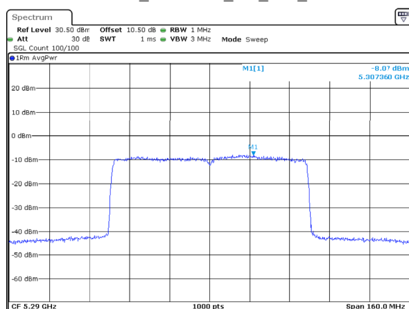
802.11ax80_5290MHz_RU_Full_Chain 2
