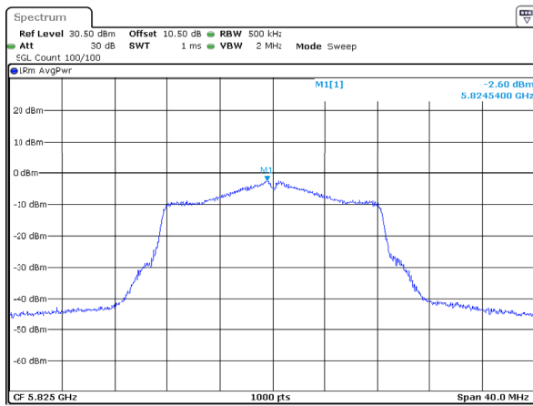
802.11a_5825MHz_Chain 1
