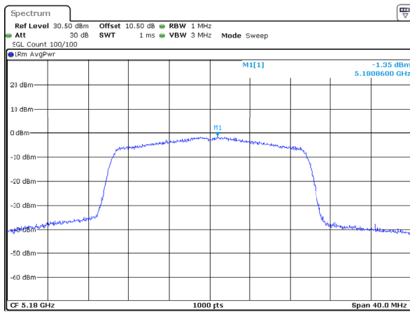
802.11ax20_5180MHz_RU_Full_Chain 1
