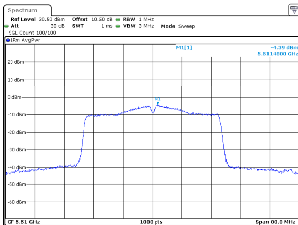
802.11ac40_5510MHz_Chain 1
