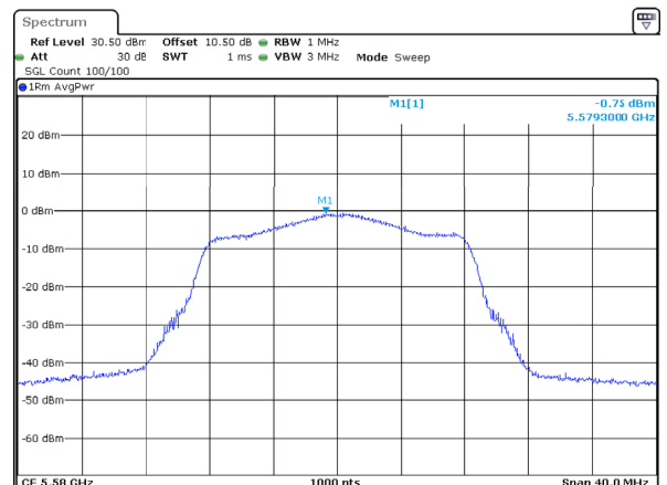
802.11a_5580MHz_Chain 2
