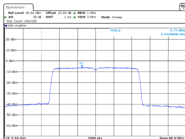
802.11ax40_5550MHz_RU_Full_Chain 2
