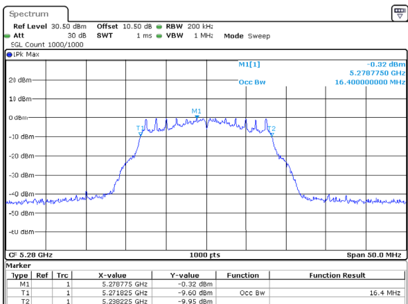
802.11a_5280MHz_Chain 2
