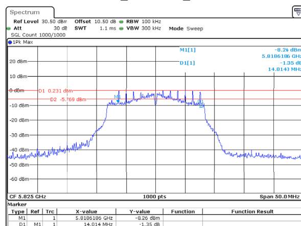
802.11a_5825MHz_Chain 2
