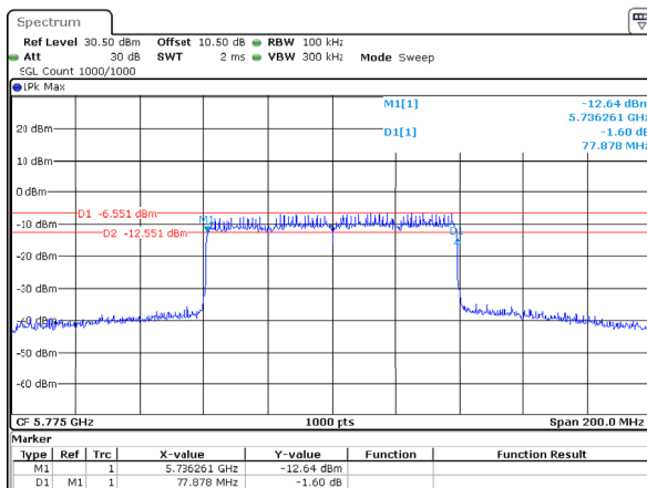
802.11ax80_5775MHz_RU_Full_Chain 1
