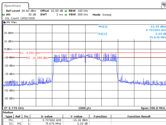
802.11ac80_5775MHz_Chain 1
