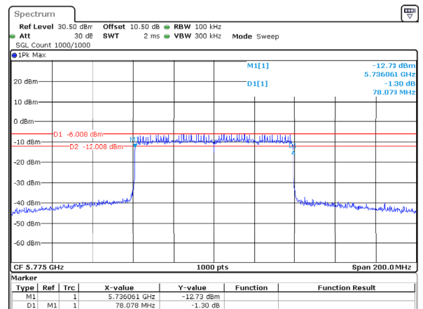
802.11ax80_5775MHz_RU_Full_Chain 2
