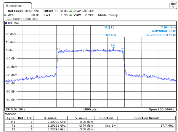
802.11ax40_5310MHz_RU_Full_Chain 1
