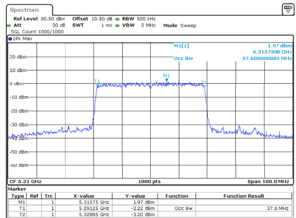
802.11ax40_5310MHz_RU_Full_Chain 2
