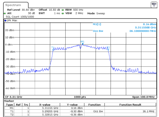
802.11ac40_5310MHz_Chain 1
