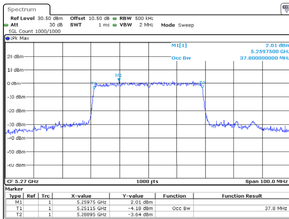
802.11ax40_5270MHz_RU_Full_Chain 1
