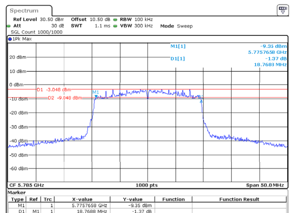
802.11ax20_5785MHz_RU_Full_Chain 1
