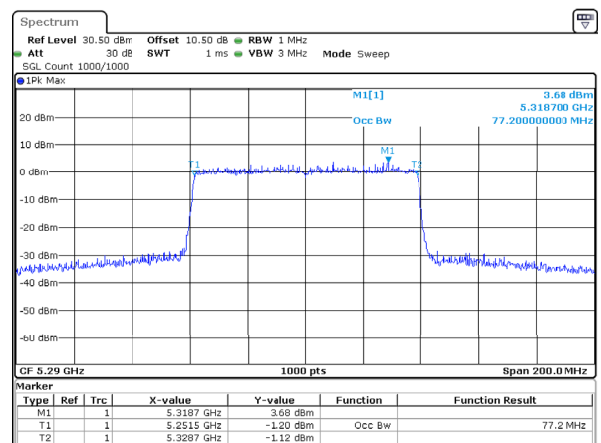
802.11ax80_5290MHz_RU_Full_Chain 2
