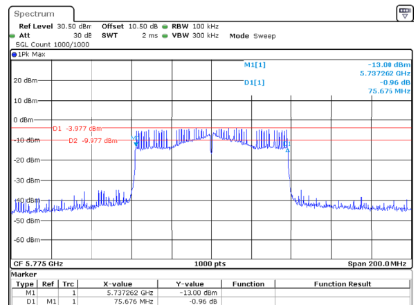
802.11ac80_5775MHz_Chain 2
