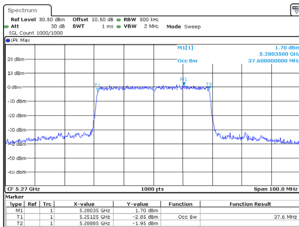
802.11ax40_5270MHz_RU_Full_Chain 2
