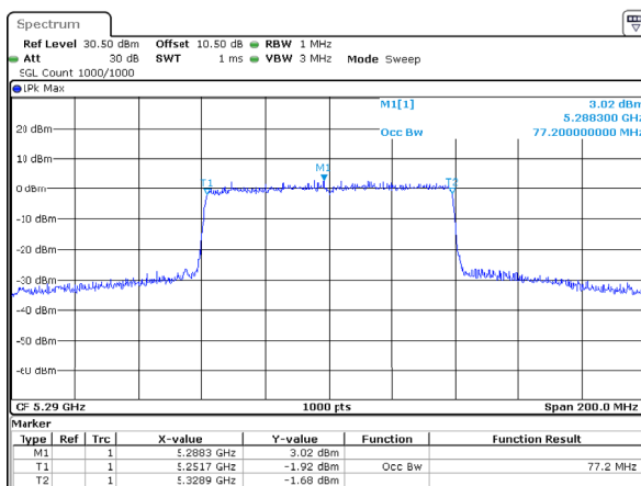
802.11ax80_5290MHz_RU_Full_Chain 1
