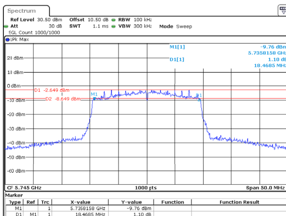
802.11ax20_5745MHz_RU_Full_Chain 1
