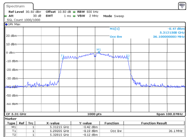
802.11ac40_5310MHz_Chain 2
