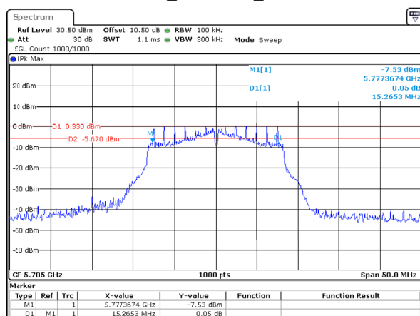
802.11a_5785MHz_Chain 2
