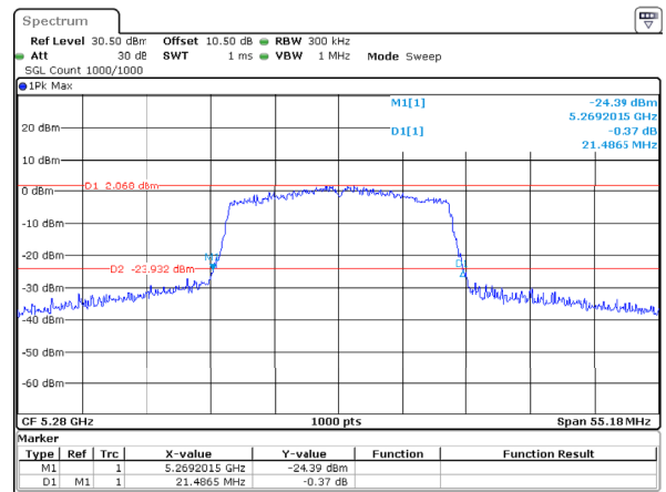
802.11ax20_5280MHz_RU_Full_Chain 1
