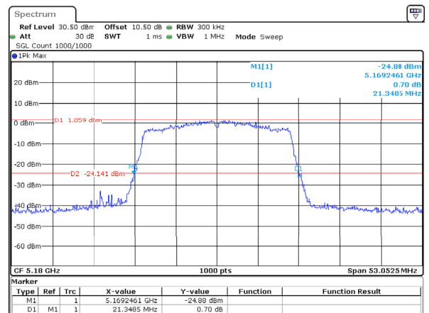
802.11ax20_5180MHz_RU_Full_Chain 2
