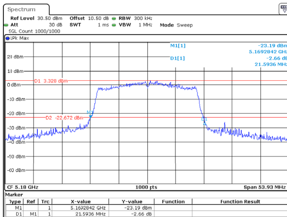
802.11ax20_5180MHz_RU_Full_Chain 1
