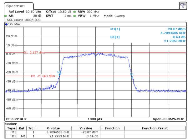
802.11ax20_5720MHz_RU_Full_Chain 2
