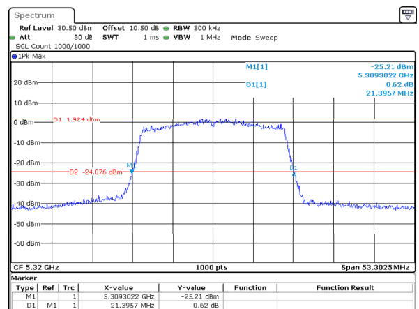
802.11ax20_5320MHz_RU_Full_Chain 2
