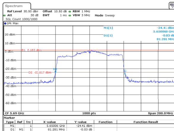
802.11ac80_5690MHz_Chain 2
