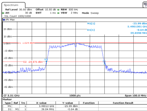
802.11ac40_5510MHz_Chain 2
