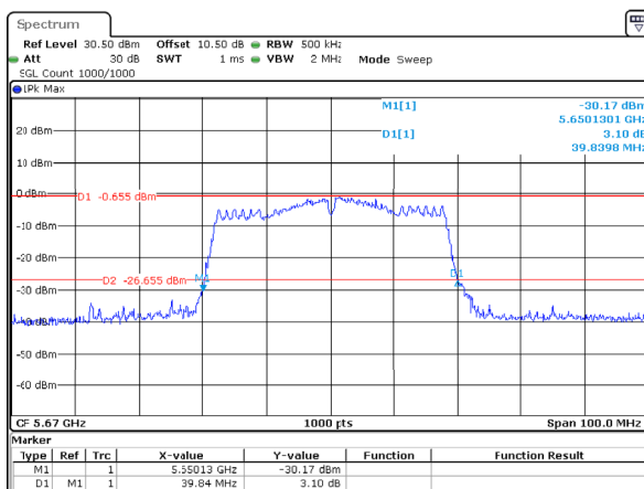
802.11ac40_5670MHz_Chain 2
