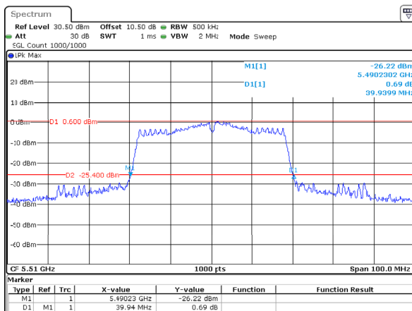
802.11ac40_5510MHz_Chain 1
