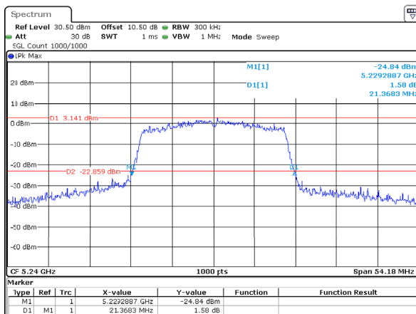
802.11ax20_5240MHz_RU_Full_Chain 1
