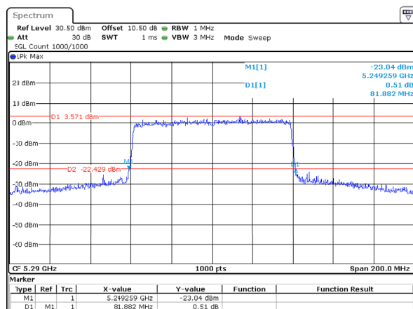
802.11ax80_5290MHz_RU_Full_Chain 1
