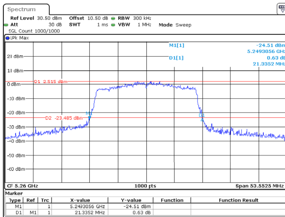
802.11ax20_5260MHz_RU_Full_Chain 1
