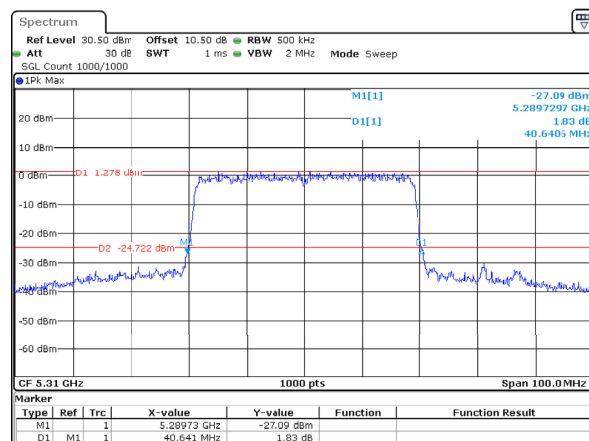
802.11ax40_5310MHz_RU_Full_Chain 2
