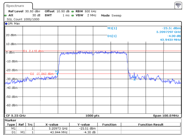
802.11ax40_5230MHz_RU_Full_Chain 1
