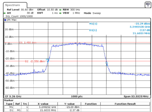
802.11ax20_5260MHz_RU_Full_Chain 2
