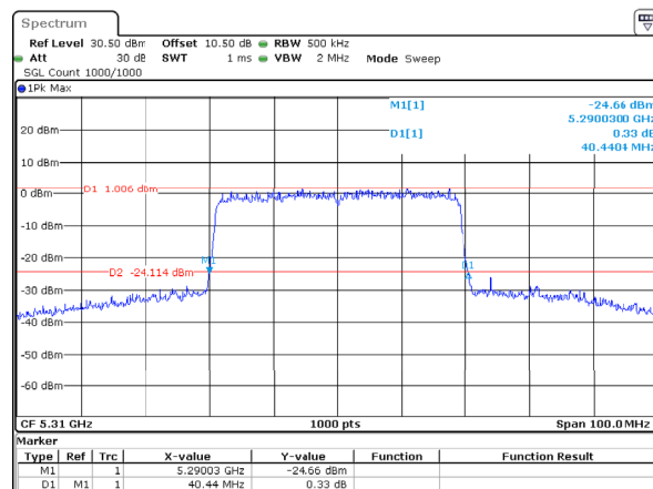
802.11ax40_5310MHz_RU_Full_Chain 1
