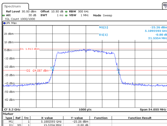
802.11ax20_5200MHz_RU_Full_Chain 2
