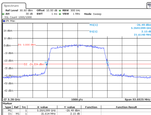
802.11ax20_5280MHz_RU_Full_Chain 2
