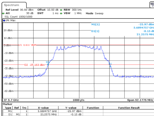
802.11a_5700MHz_Chain 2
