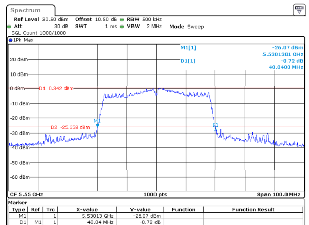
802.11ac40_5550MHz_Chain 1
