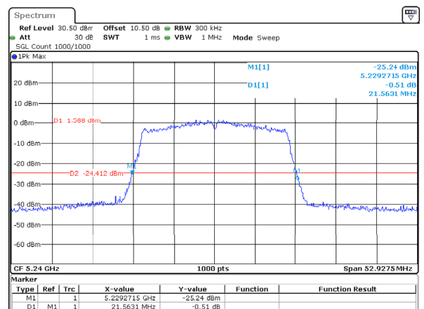
802.11ax20_5240MHz_RU_Full_Chain 2
