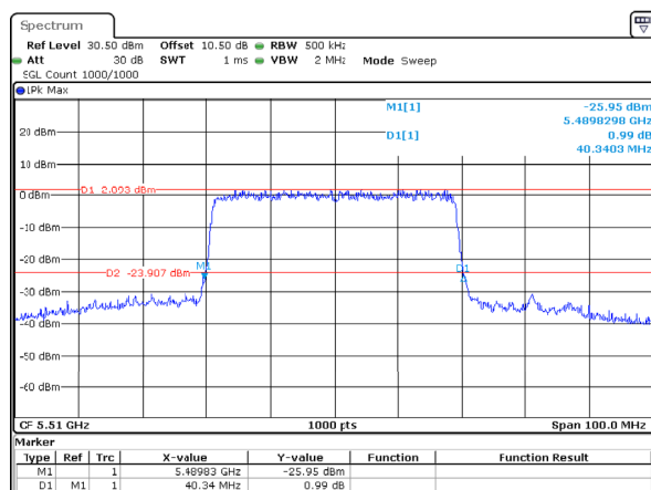
802.11ax40_5510MHz_RU_Full_Chain 2
