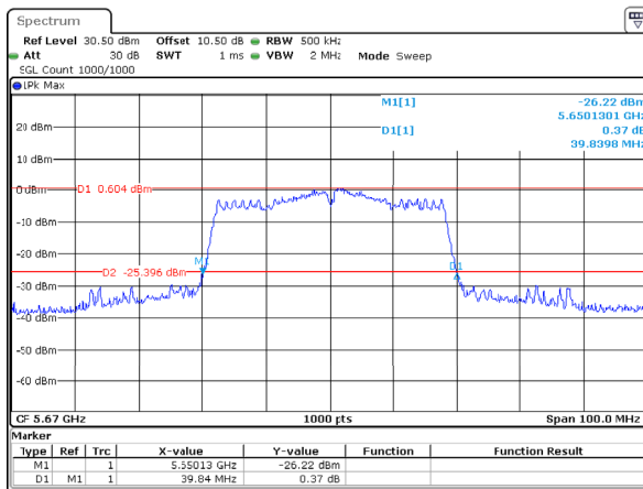
802.11ac40_5670MHz_Chain 1
