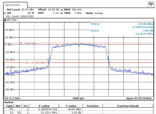
802.11ax20_5200MHz_RU_Full_Chain 1
