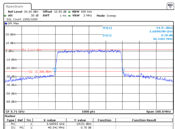
802.11ax40_5710MHz_RU_Full_Chain 1
