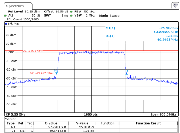
802.11ax40_5550MHz_RU_Full_Chain 1
