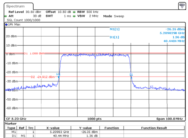
802.11ax40_5230MHz_RU_Full_Chain 2
