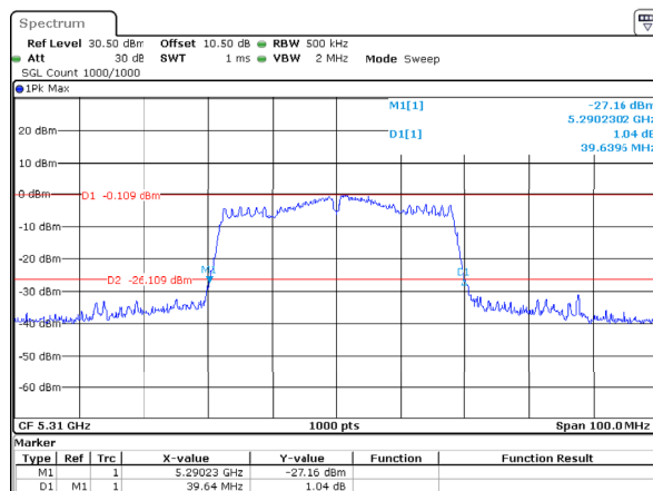
802.11ac40_5310MHz_Chain 1
