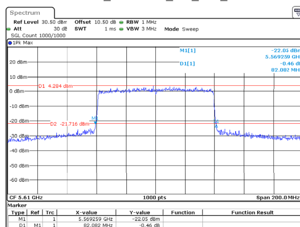
802.11ax80_5610MHz_RU_Full_Chain 1
