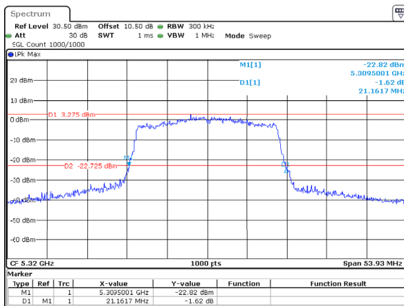
802.11ax20_5320MHz_RU_Full_Chain 1
