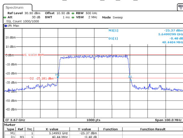
802.11ax40_5670MHz_RU_Full_Chain 2
