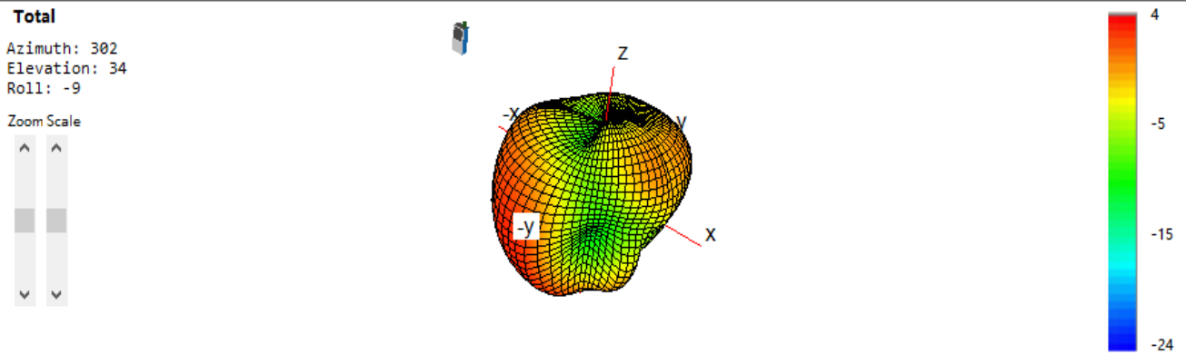
3D Antenna pattern
