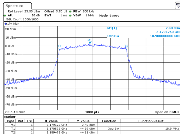
802.11ax20_5180MHz_RU_Full
