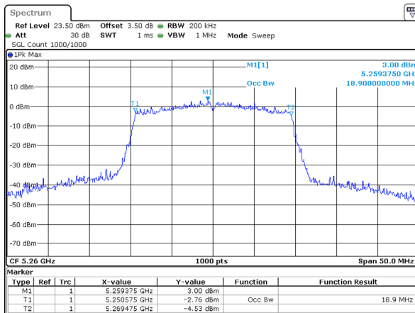
802.11ax20_5260MHz_RU_Full
