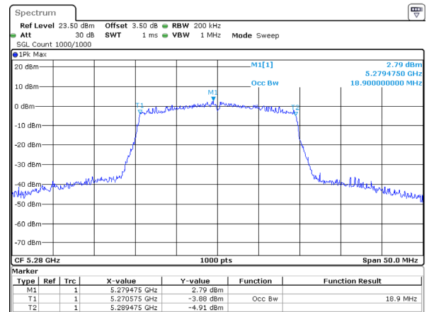
802.11ax20_5280MHz_RU_Full
