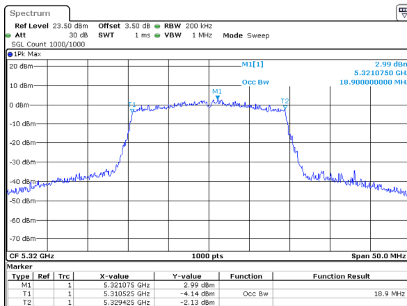
802.11ax20_5320MHz_RU_Full
