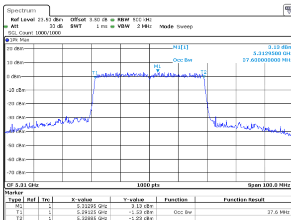
802.11ax40_5310MHz_RU_Full
