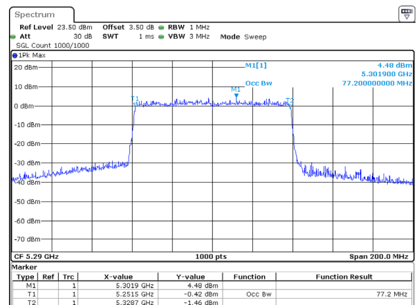
802.11ax80_5290MHz_RU_Full
