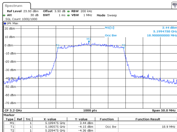
802.11ax20_5200MHz_RU_Full
