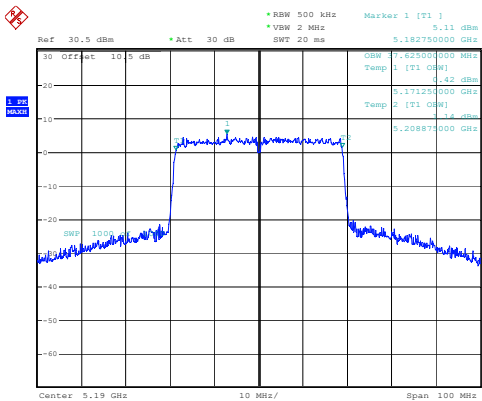
802.11ax40_5190MHz_RU_Full
