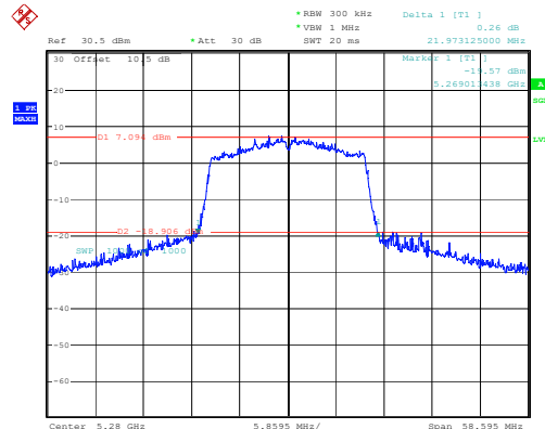
802.11ax20_5280MHz_RU_Full
