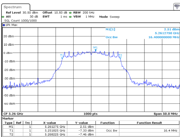
802.11a_5260MHz
