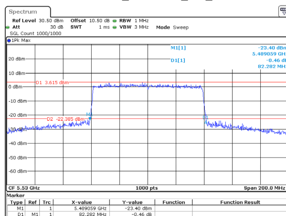
802.11ax80_5530MHz_RU_Full
