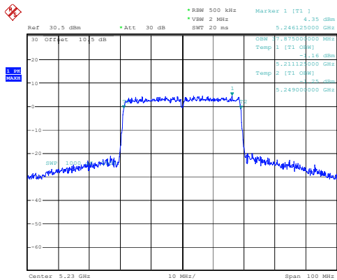
802.11ax40_5230MHz_RU_Full
