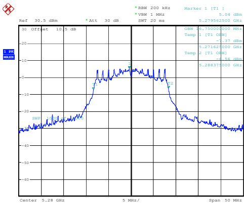
802.11a_5280MHz
