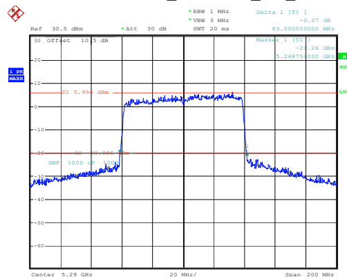
802.11ax80_5290MHz_RU_Full
