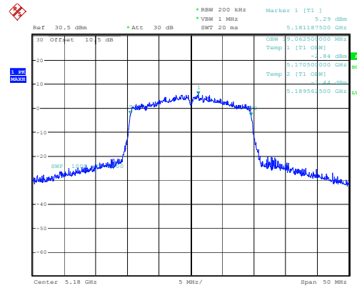
802.11ax20_5180MHz_RU_Full
