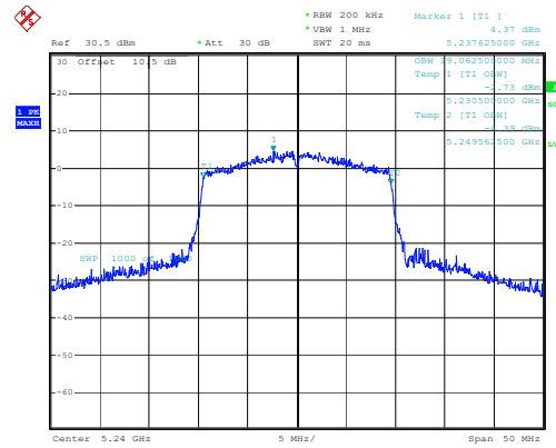
802.11ax20_5240MHz_RU_Full
