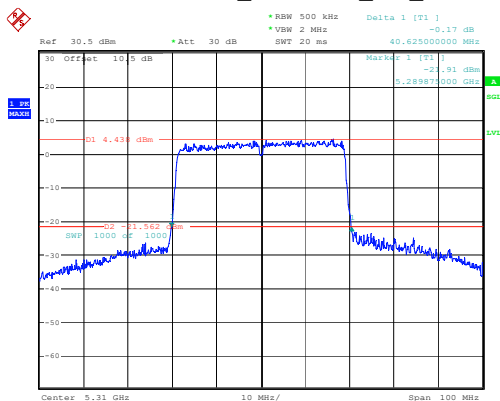
802.11ax40_5310MHz_RU_Full
