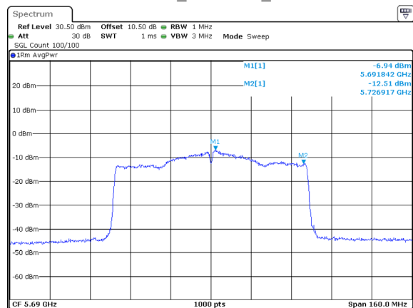
802.11ac80_5690MHz_Chain 2
