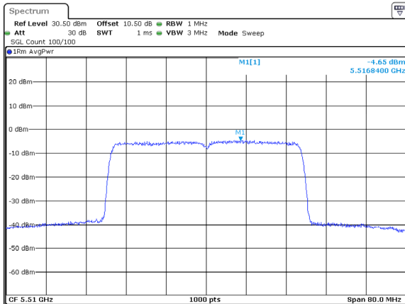
802.11ax40_5510MHz_RU_Full_Chain 2
