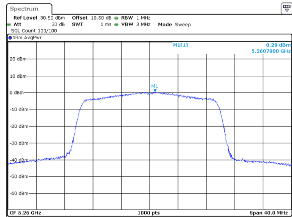
802.11ax20_5260MHz_RU_Full_Chain 2
