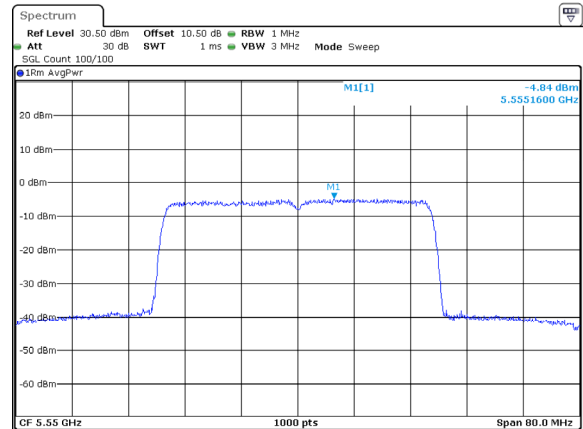
802.11ax40_5550MHz_RU_Full_Chain 2
