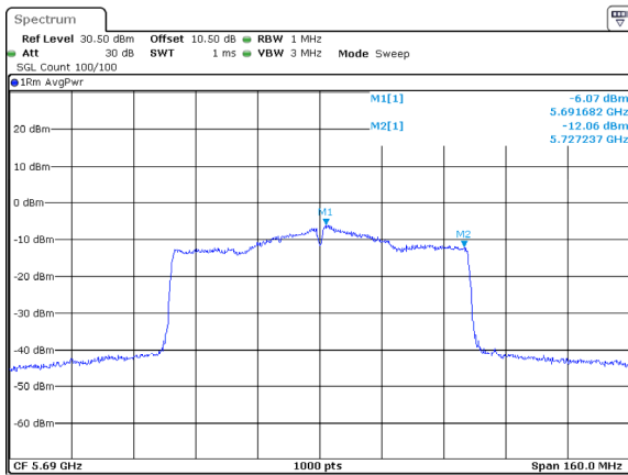
802.11ac80_5690MHz_Chain 1
