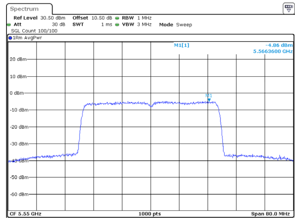
802.11ax40_5550MHz_RU_Full_Chain 1
