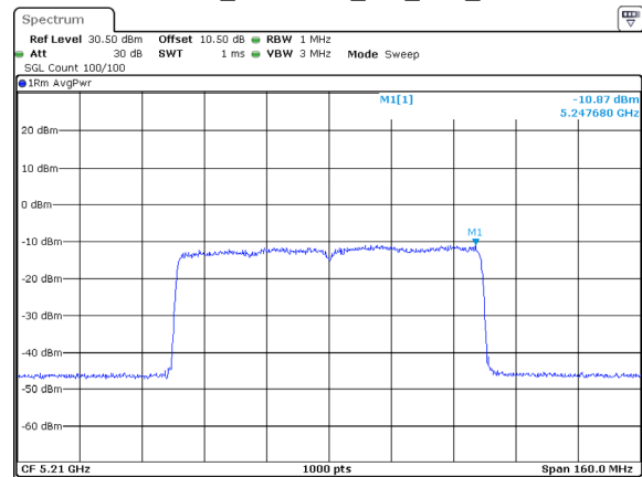
802.11ax80_5210MHz_RU_Full_Chain 2
