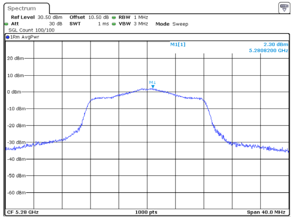
802.11a_5280MHz_Chain 1
