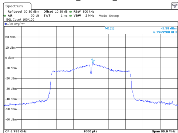
802.11ac40_5795MHz_Chain 1
