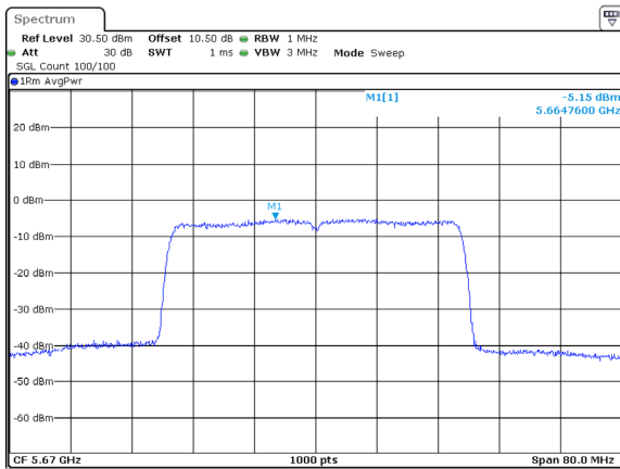
802.11ax40_5670MHz_RU_Full_Chain 2
