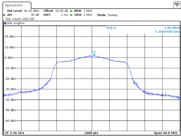
802.11a_5260MHz_Chain 1
