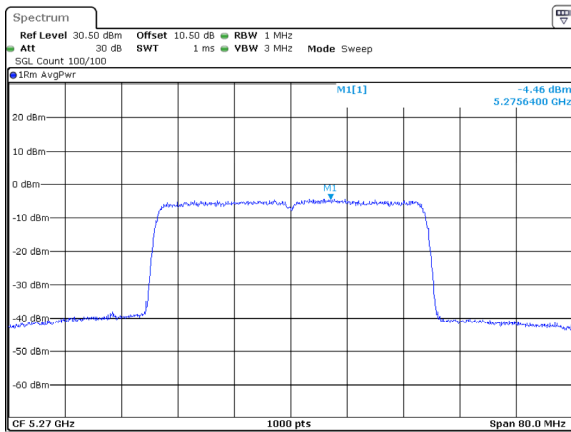
802.11ax40_5270MHz_RU_Full_Chain 2
