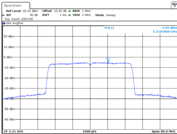
802.11ax40_5510MHz_RU_Full_Chain 1
