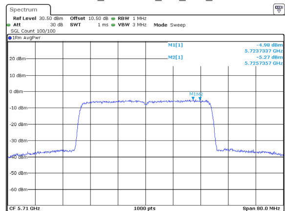
802.11ax40_5710MHz_RU_Full_Chain 1
