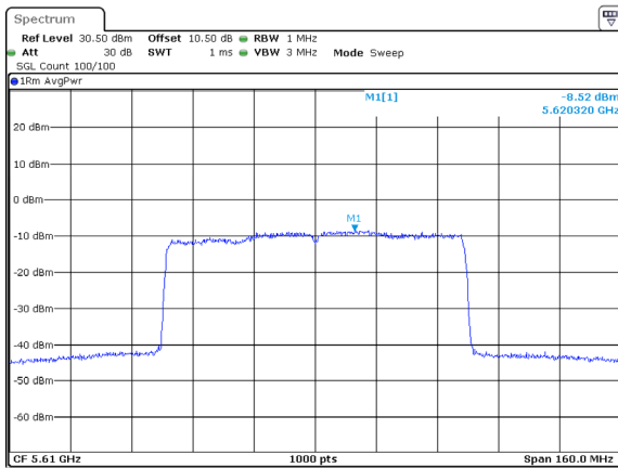
802.11ax80_5610MHz_RU_Full_Chain 2
