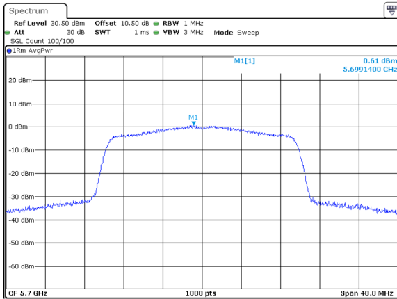
802.11ax20_5700MHz_RU_Full_Chain 1
