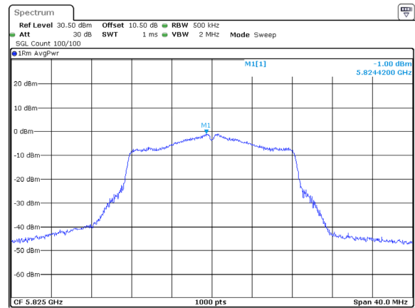
802.11a_5825MHz_Chain 2
