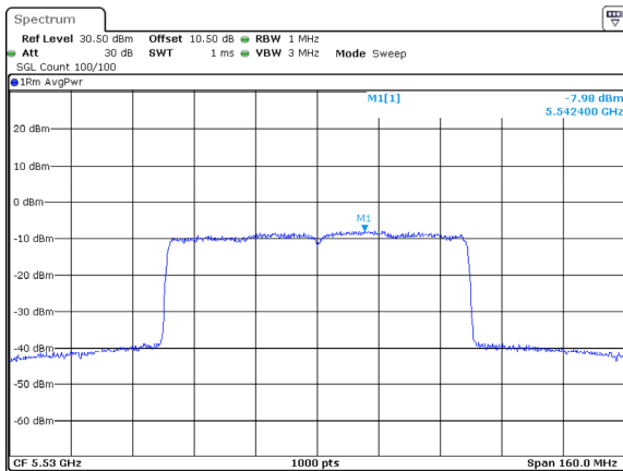
802.11ax80_5530MHz_RU_Full_Chain 1
