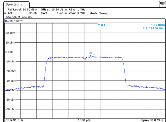
802.11ax40_5310MHz_RU_Full_Chain 1
