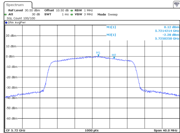
802.11ax20_5720MHz_RU_Full_Chain 1
