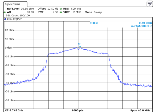
802.11a_5745MHz_Chain 2
