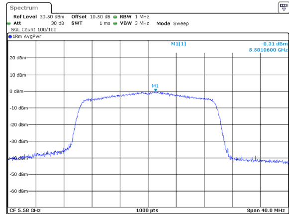
802.11ax20_5580MHz_RU_Full_Chain 2
