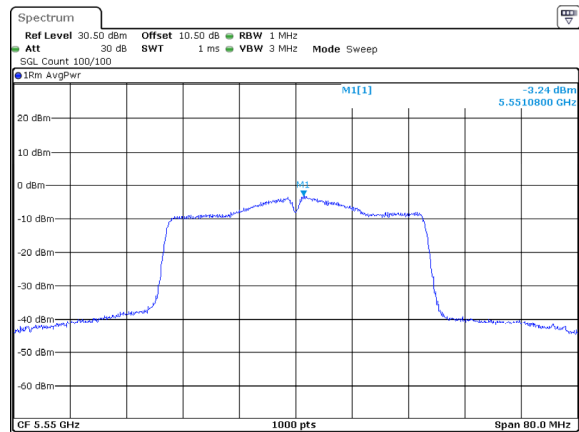
802.11ac40_5550MHz_Chain 1
