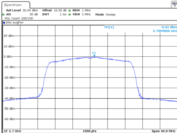
802.11ax20_5700MHz_RU_Full_Chain 2
