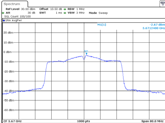
802.11ac40_5670MHz_Chain 1
