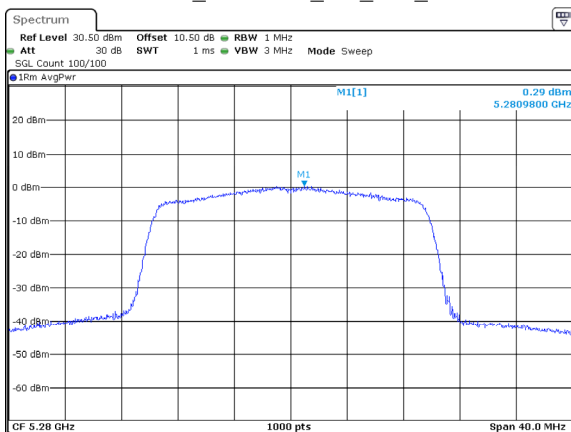
802.11ax20_5280MHz_RU_Full_Chain 2
