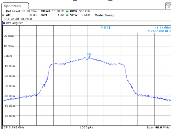
802.11ac20_5745MHz_Chain 1
