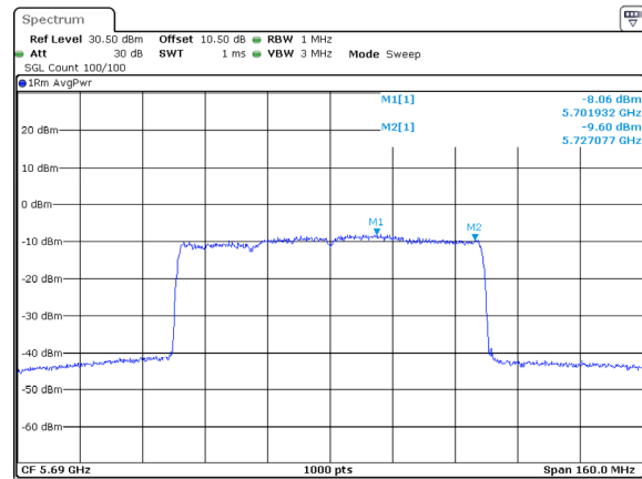
802.11ax80_5690MHz_RU_Full_Chain 2
