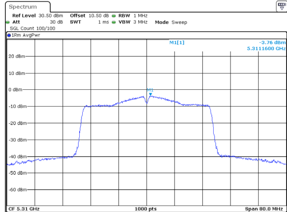
802.11ac40_5310MHz_Chain 1
