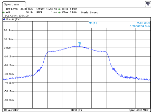
802.11a_5700MHz_Chain 1
