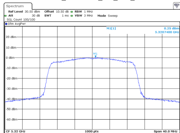
802.11ax20_5320MHz_RU_Full_Chain 2
