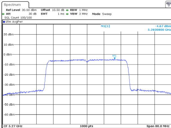
802.11ax40_5270MHz_RU_Full_Chain 1
