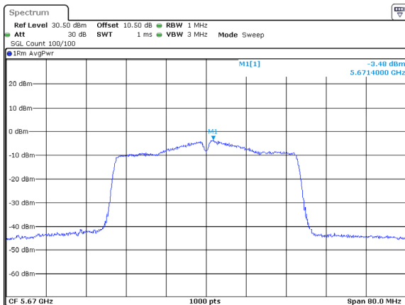
802.11ac40_5670MHz_Chain 2
