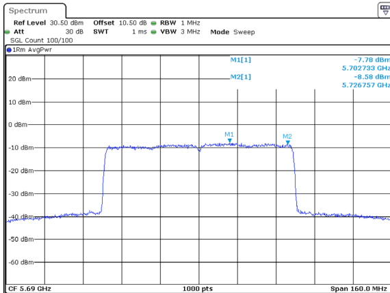
802.11ax80_5690MHz_RU_Full_Chain 1
