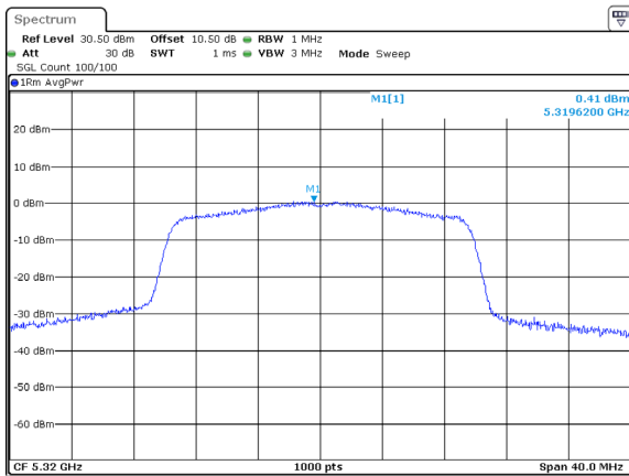
802.11ax20_5320MHz_RU_Full_Chain 1
