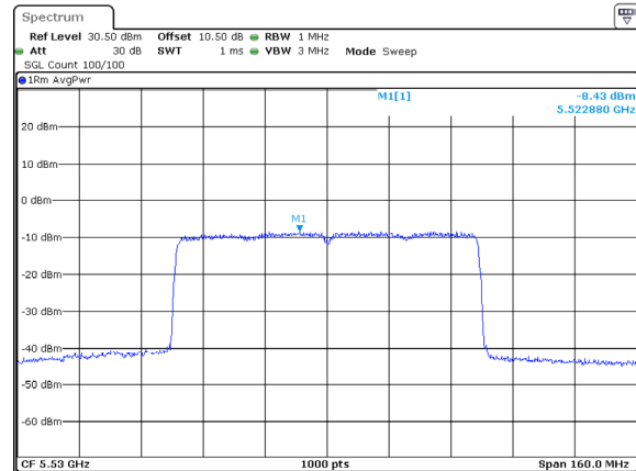
802.11ax80_5530MHz_RU_Full_Chain 2
