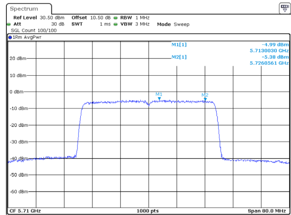
802.11ax40_5710MHz_RU_Full_Chain 2
