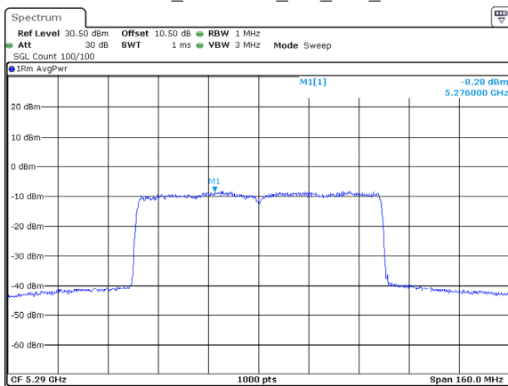
802.11ax80_5290MHz_RU_Full_Chain 1
