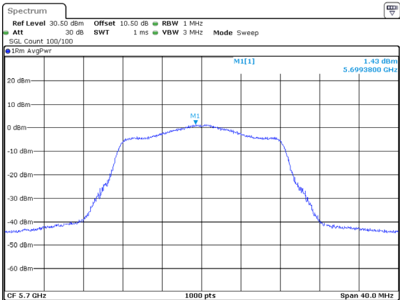
802.11a_5700MHz_Chain 2
