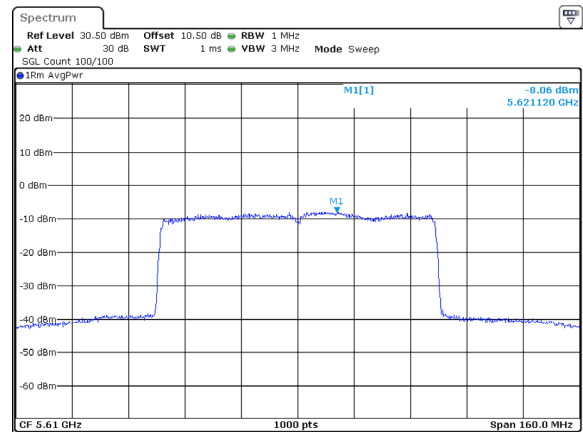
802.11ax80_5610MHz_RU_Full_Chain 1
