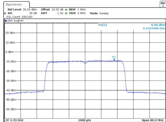
802.11ax40_5230MHz_RU_Full_Chain 1
