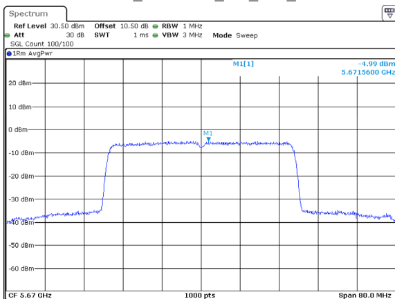
802.11ax40_5670MHz_RU_Full_Chain 1
