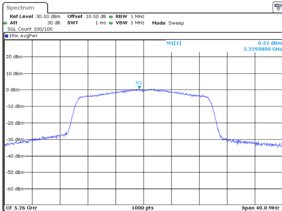
802.11ax20_5260MHz_RU_Full_Chain 1
