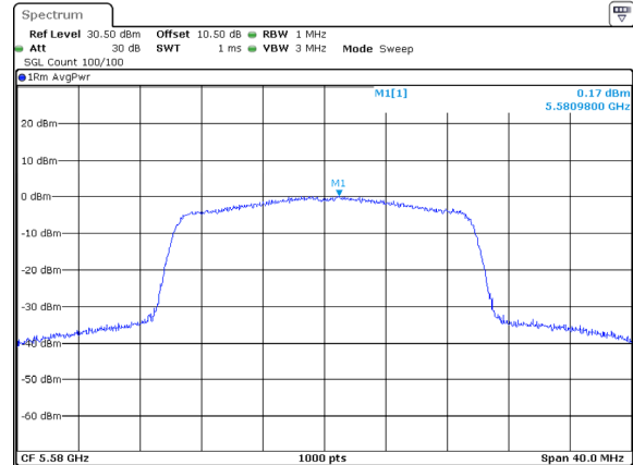
802.11ax20_5580MHz_RU_Full_Chain 1
