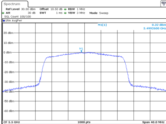
802.11ax20_5500MHz_RU_Full_Chain 1
