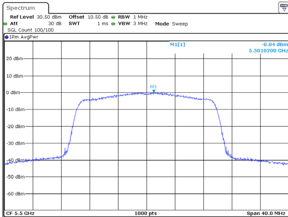
802.11ax20_5500MHz_RU_Full_Chain 2
