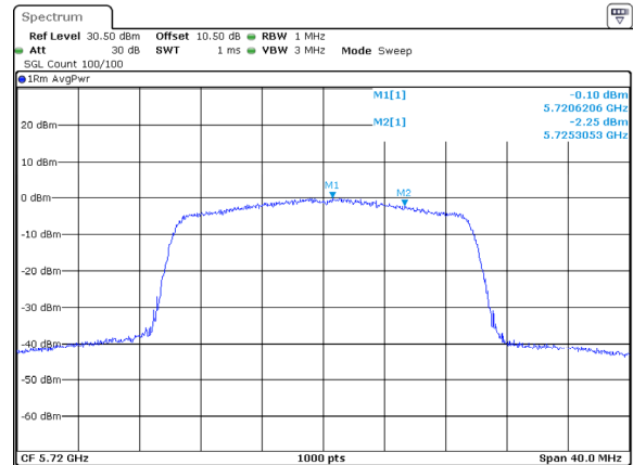
802.11ax20_5720MHz_RU_Full_Chain 2
