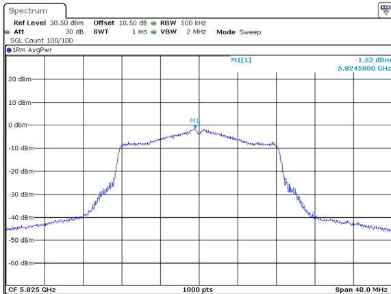
802.11a_5825MHz_Chain 1
