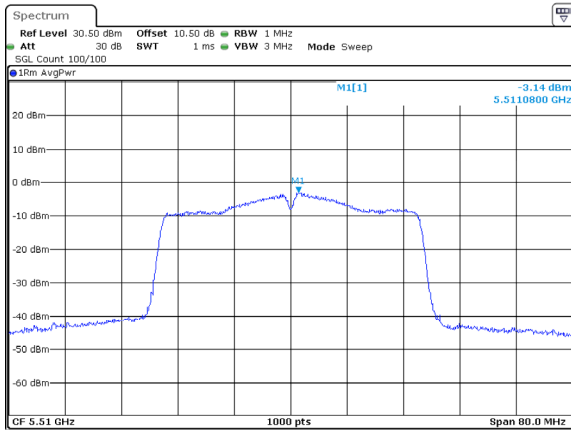
802.11ac40_5510MHz_Chain 2
