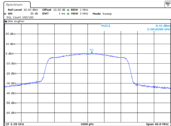
802.11ax20_5280MHz_RU_Full_Chain 1
