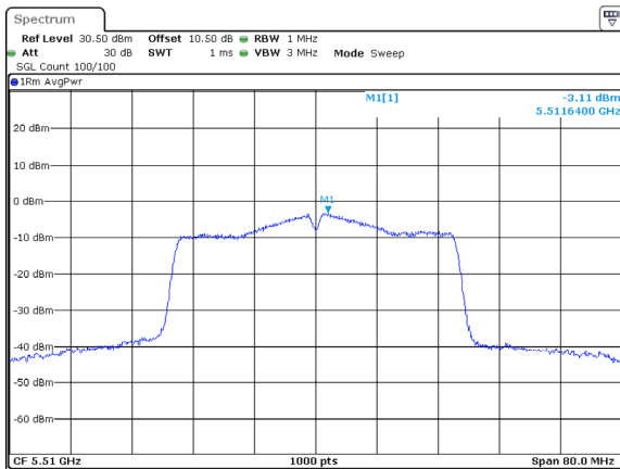
802.11ac40_5510MHz_Chain 1
