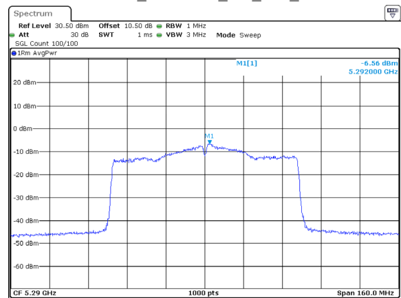
802.11ax80_5290MHz_RU_Full_Chain 2
