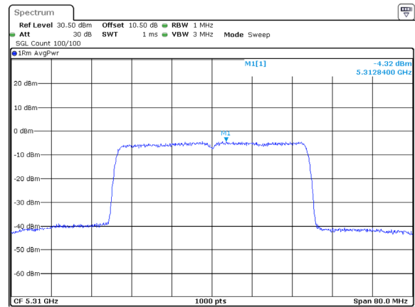
802.11ax40_5310MHz_RU_Full_Chain 2
