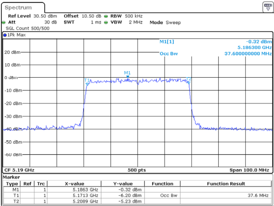
802.11ax40_5190MHz_RU_Full_Chain 2
