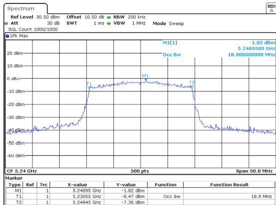
802.11ax20_5240MHz_RU_Full_Chain 1
