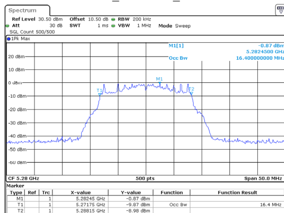
802.11a_5280MHz_Chain 2
