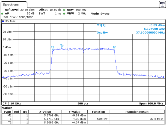
802.11ax40_5190MHz_RU_Full_Chain 1
