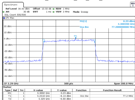
802.11ax80_5290MHz_RU_Full_Chain 1
