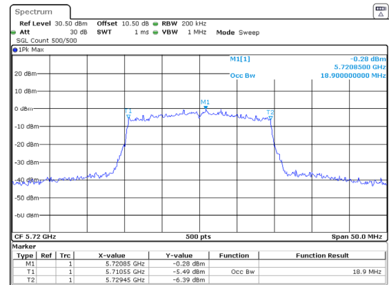
802.11ax20_5720MHz_RU_Full_Chain 1
