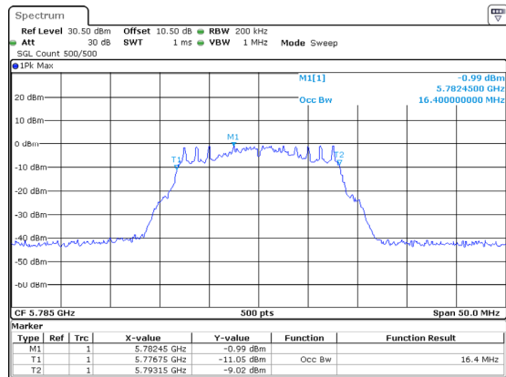
802.11a_5785MHz_Chain 2
