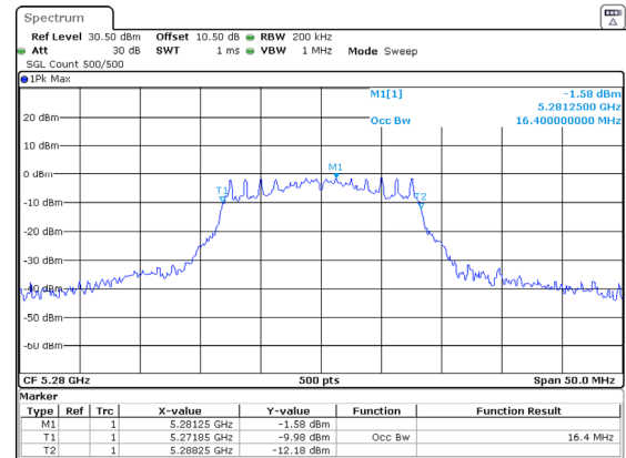
802.11a_5280MHz_Chain 1
