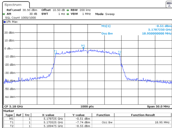
802.11ax20_5180MHz_RU_Full_Chain 1
