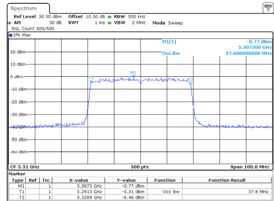
802.11ax40_5310MHz_RU_Full_Chain 2
