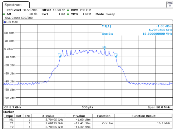
802.11a_5700MHz_Chain 2
