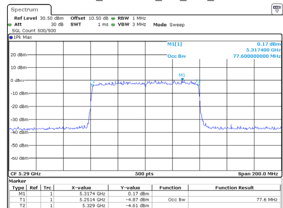
802.11ax80_5290MHz_RU_Full_Chain 2
