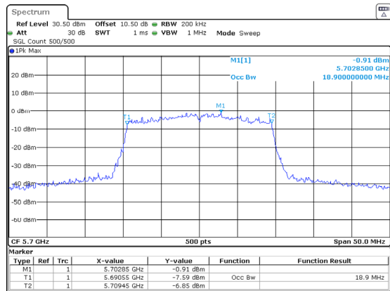
802.11ax20_5700MHz_RU_Full_Chain 1
