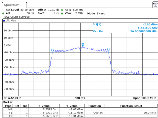
802.11ac40_5550MHz_Chain 1
