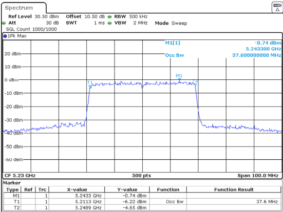
802.11ax40_5230MHz_RU_Full_Chain 1
