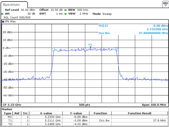
802.11ax40_5230MHz_RU_Full_Chain 2
