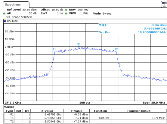
802.11ax20_5500MHz_RU_Full_Chain 1
