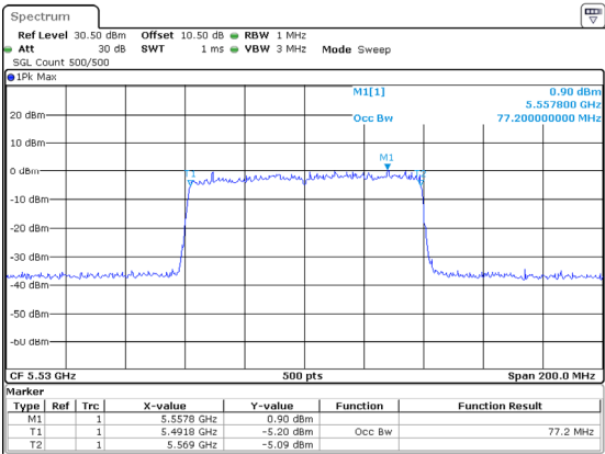
802.11ax80_5530MHz_RU_Full_Chain 2
