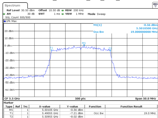
802.11ax20_5500MHz_RU_Full_Chain 2
