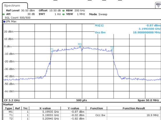
802.11ax20_5200MHz_RU_Full_Chain 2
