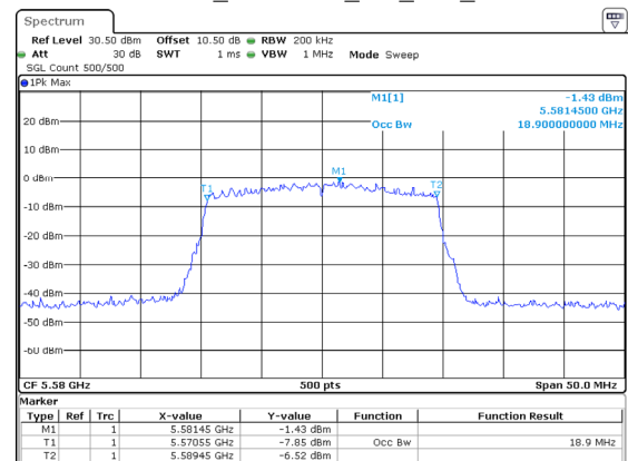
802.11ax20_5580MHz_RU_Full_Chain 2
