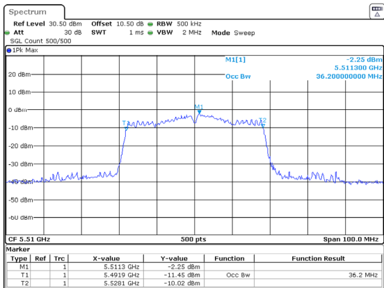
802.11ac40_5510MHz_Chain 1
