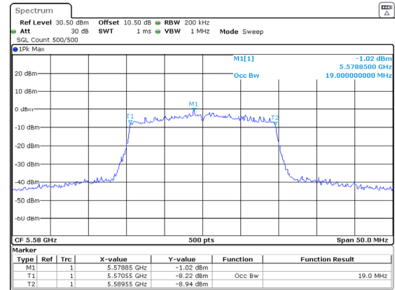
802.11ax20_5580MHz_RU_Full_Chain 1
