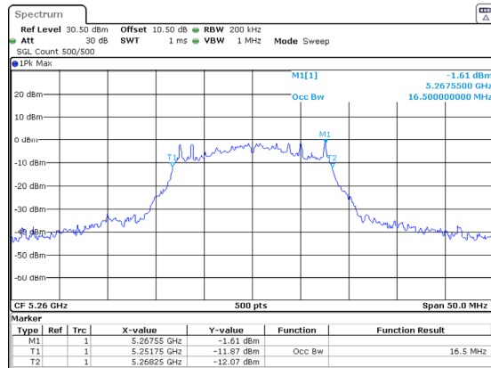
802.11a_5260MHz_Chain 1
