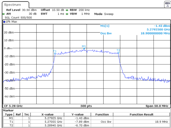
802.11ax20_5280MHz_RU_Full_Chain 1
