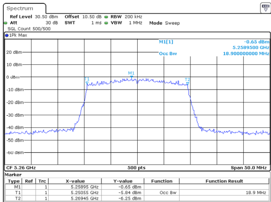
802.11ax20_5260MHz_RU_Full_Chain 2
