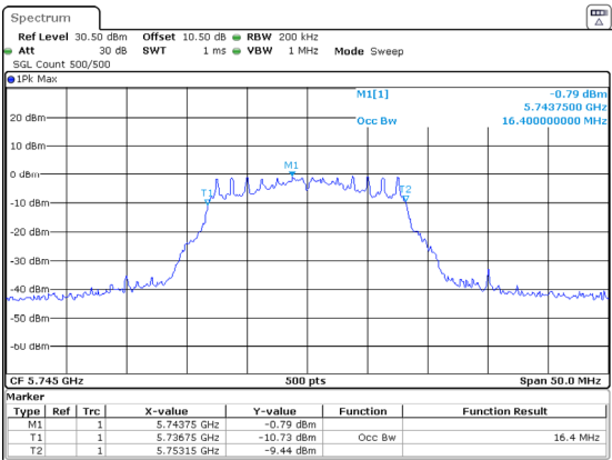
802.11a_5745MHz_Chain 1
