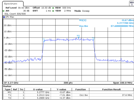
802.11ax40_5270MHz_RU_Full_Chain 1
