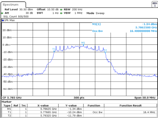
802.11a_5785MHz_Chain 1
