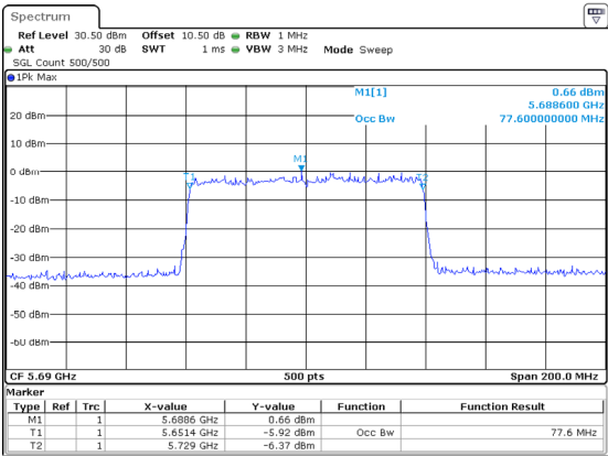
802.11ax80_5690MHz_RU_Full_Chain 2
