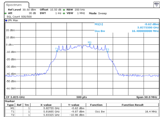
802.11a_5825MHz_Chain 2
