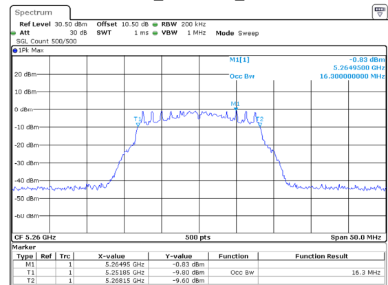
802.11a_5260MHz_Chain 2
