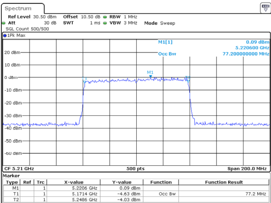
802.11ax80_5210MHz_RU_Full_Chain 2
