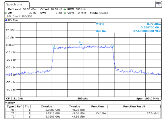
802.11ax40_5310MHz_RU_Full_Chain 1
