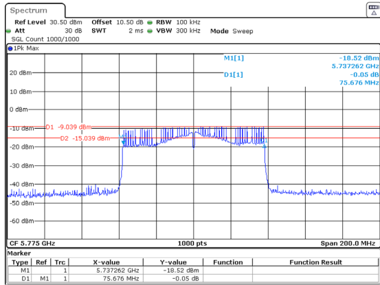
802.11ac80_5775MHz_Chain 1
