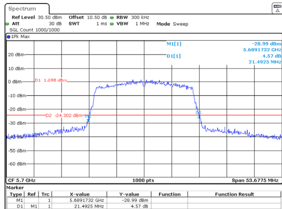
802.11ax20_5700MHz_RU_Full_Chain 1
