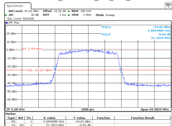
802.11ax20_5580MHz_RU_Full_Chain 2
