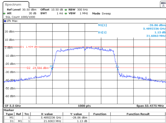
802.11ax20_5500MHz_RU_Full_Chain 1
