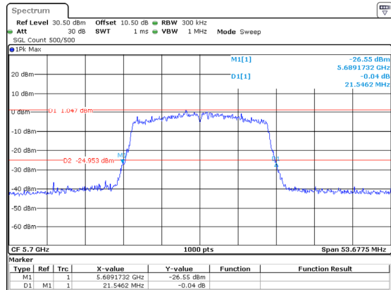
802.11ax20_5700MHz_RU_Full_Chain 2
