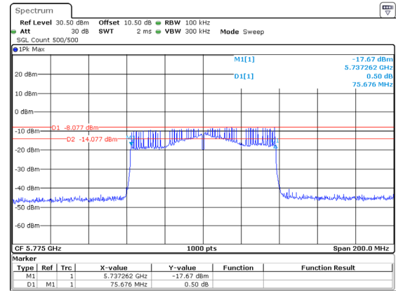
802.11ac80_5775MHz_Chain 2
