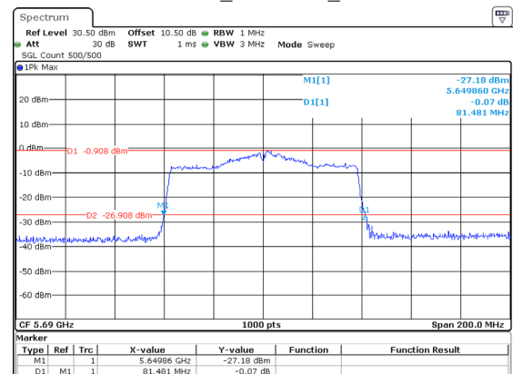
802.11ac80_5690MHz_Chain 2
