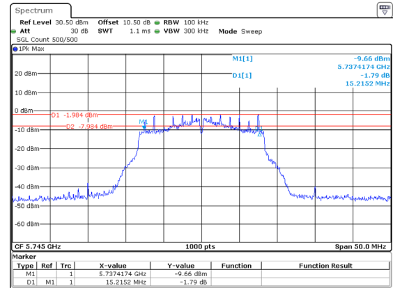
802.11ac20_5745MHz_Chain 2
