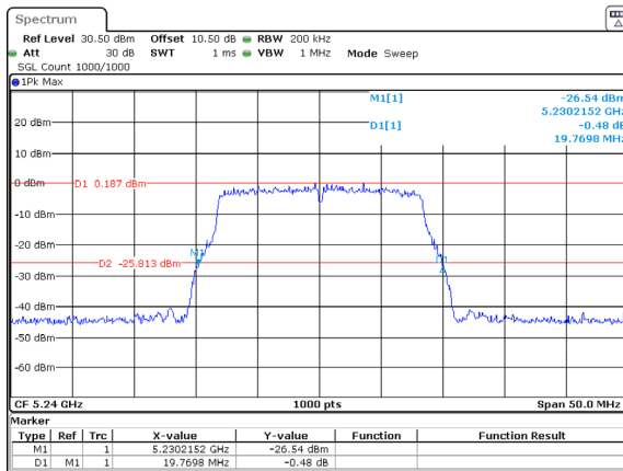
802.11a_5240MHz_Chain 1
