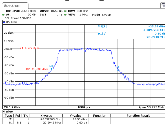
802.11a_5200MHz_Chain 2
