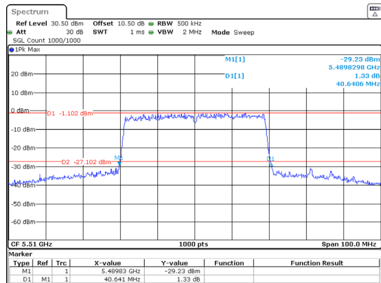
802.11ax40_5510MHz_RU_Full_Chain 1
