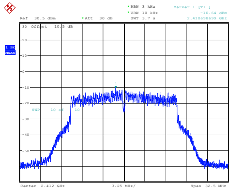
802.11g_2412MHz_Chain 2
