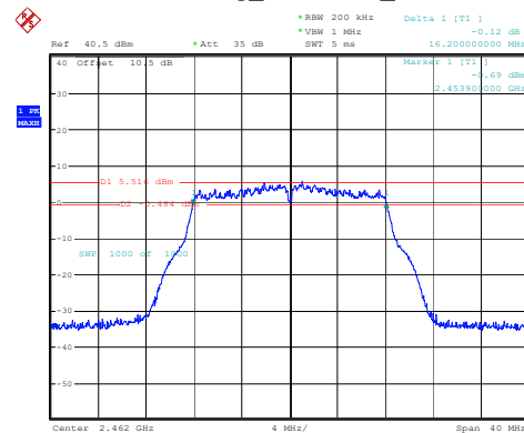
802.11g_2462MHz_Chain 2
