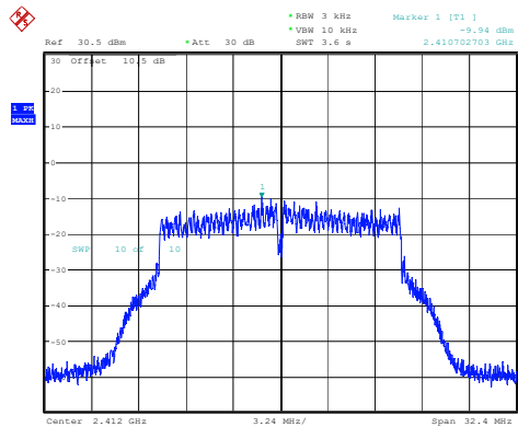
802.11g_2412MHz_Chain 1
