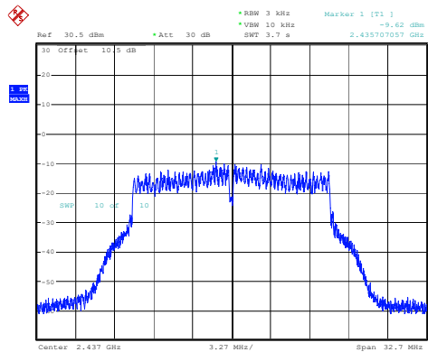
802.11g_2437MHz_Chain 1
