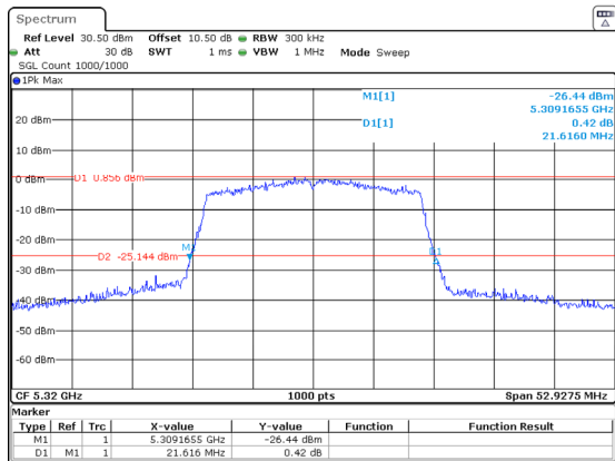
802.11ax20_5320MHz_RU_Full_Chain 1
