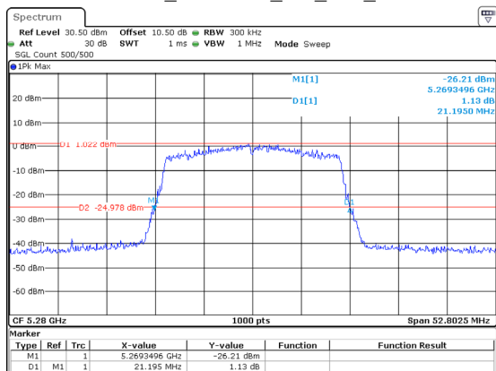
802.11ax20_5280MHz_RU_Full_Chain 2
