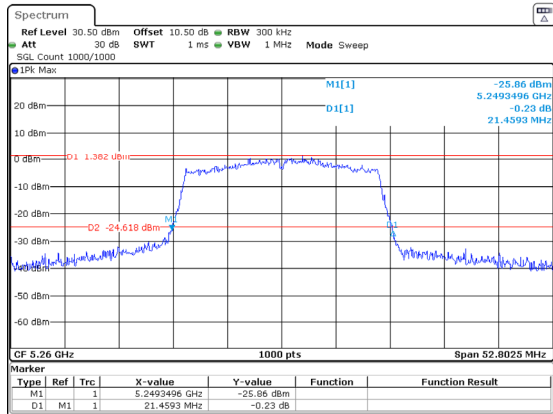
802.11ax20_5260MHz_RU_Full_Chain 1
