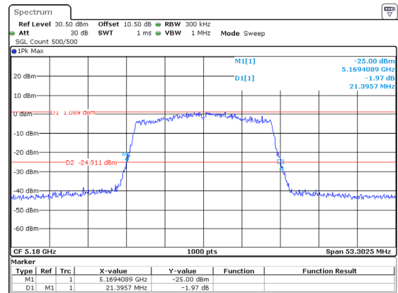
802.11ax20_5180MHz_RU_Full_Chain 2
