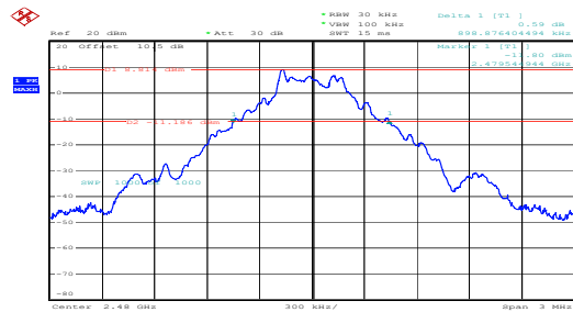
GFSK_High 0.899MHz
