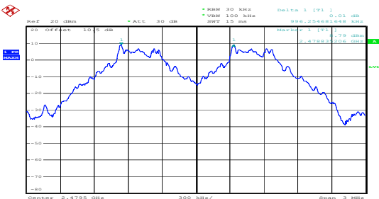
GFSK_High 0.996MHz
