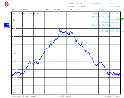
GFSK_Middle
