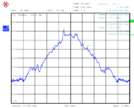
GFSK_Low
