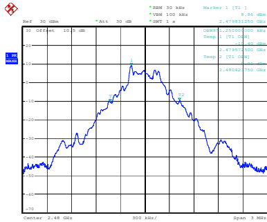
GFSK_High
