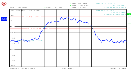
8DPSK_Middle 1.243MHz
