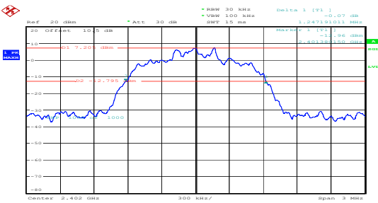
8DPSK_Low 1.247MHz
