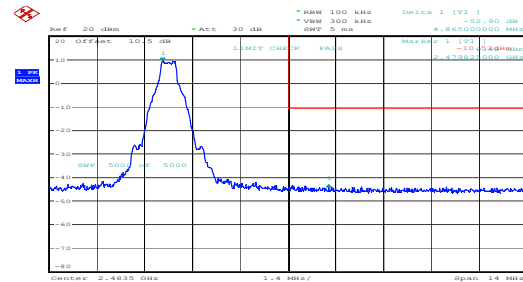
GFSK_High
