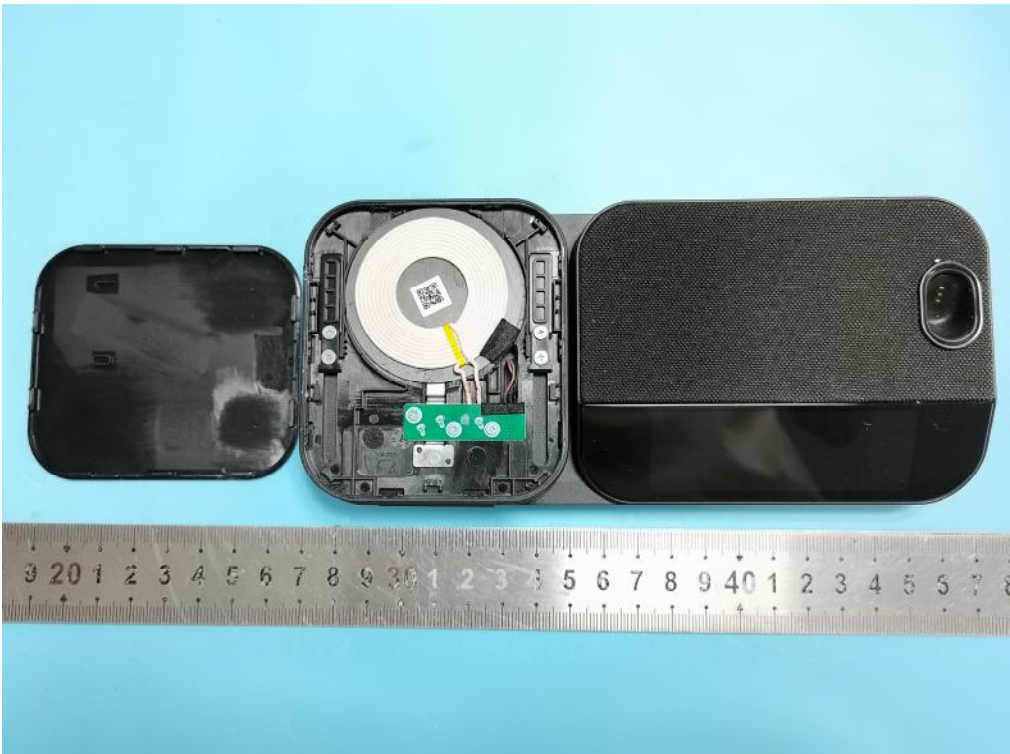
WPT Coil Antenna
