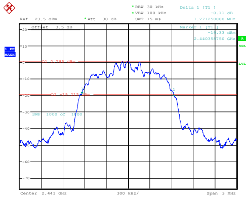
2DH1_Middle 1.271MHz
