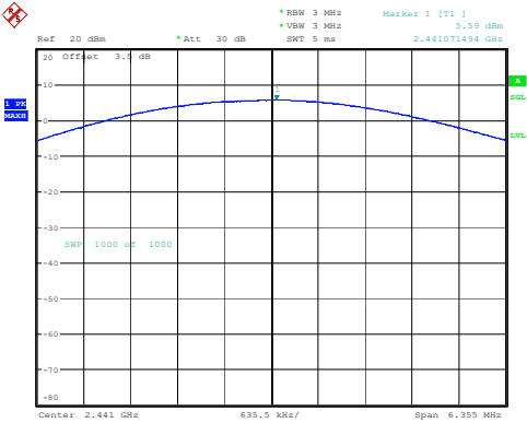
2DH1_Middle 5.59dBm
