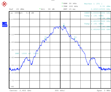
DH1_Low 0.870MHz
