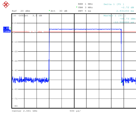
DH5_Hopping 2.931ms
