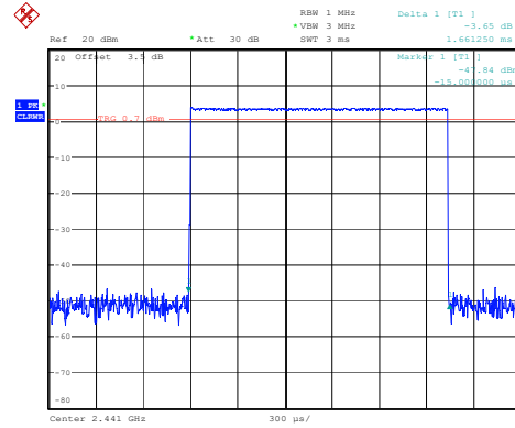
DH3_Hopping 1.661ms
