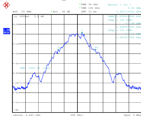
DH1_Middle 0.870MHz
