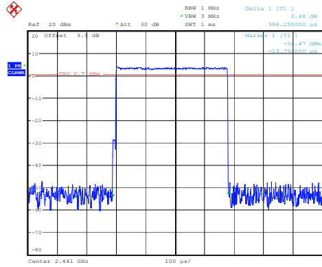
DH1_Hopping 0.396ms
