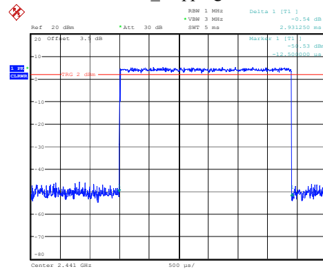
2DH5_Hopping 2.931ms
