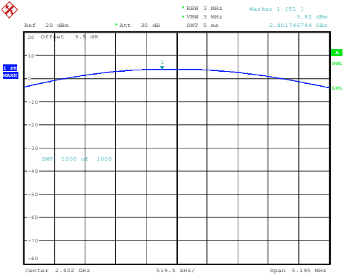
DH1_Low 3.82dBm
