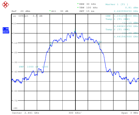
2DH1_Middle 1.151MHz
