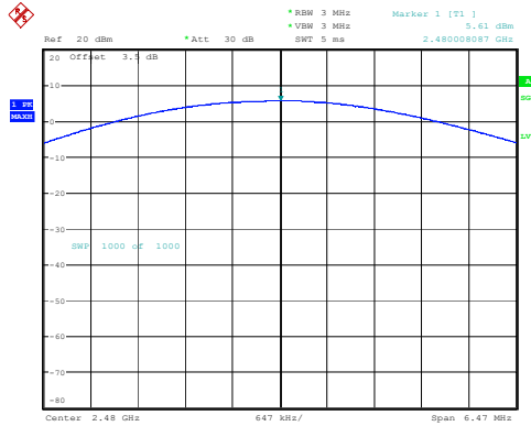
2DH1_High 5.61dBm
