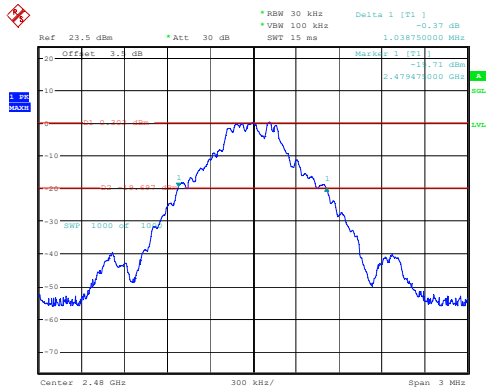
DH1_High 1.039MHz
