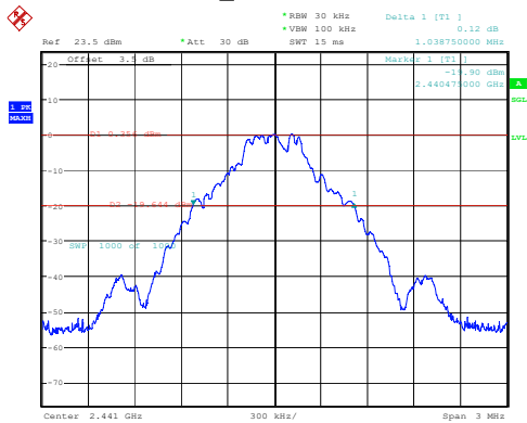
DH1_Middle 1.039MHz
