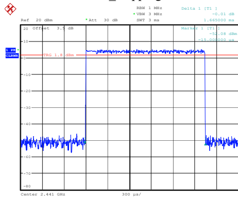
2DH3_Hopping 1.665ms
