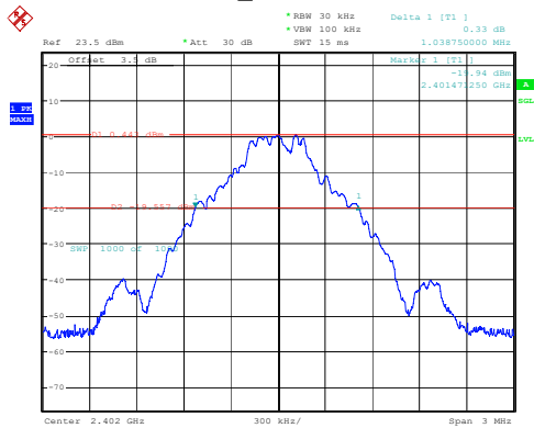
DH1_Low 1.039MHz
