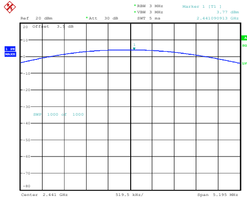
DH1_Middle 3.77dBm
