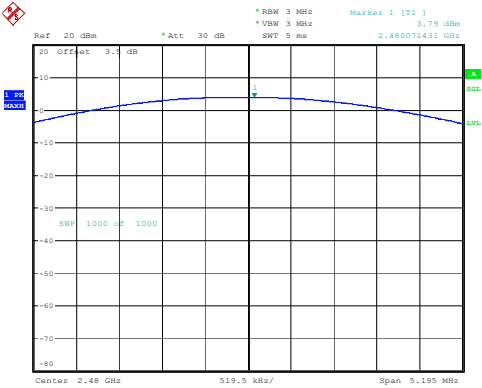
DH1_High 3.79dBm
