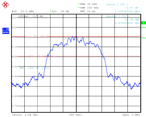
2DH1_High 1.294MHz
