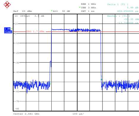
2DH1_Hopping 0.406ms
