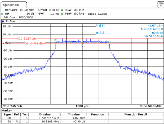
802.11a_5745MHz
