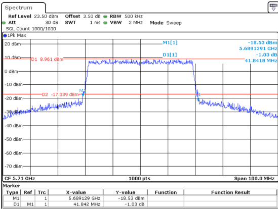
802.11ax40_5710MHz_RU_Full
