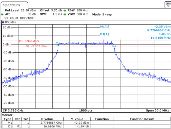
802.11a_5785MHz
