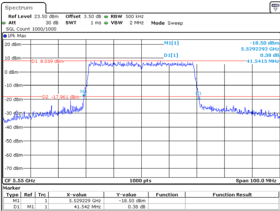
802.11ax40_5550MHz_RU_Full
