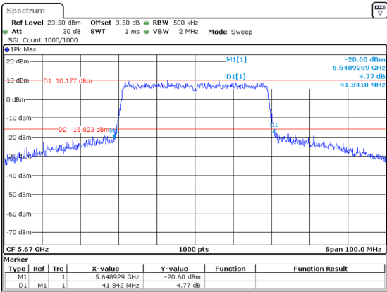
802.11ax40_5670MHz_RU_Full
