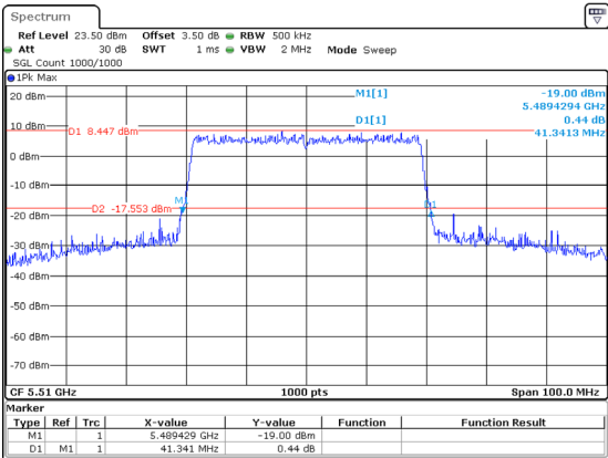
802.11ax40_5510MHz_RU_Full
