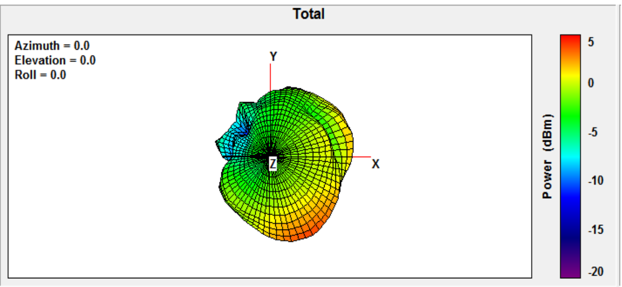
3D Antenna pattern
