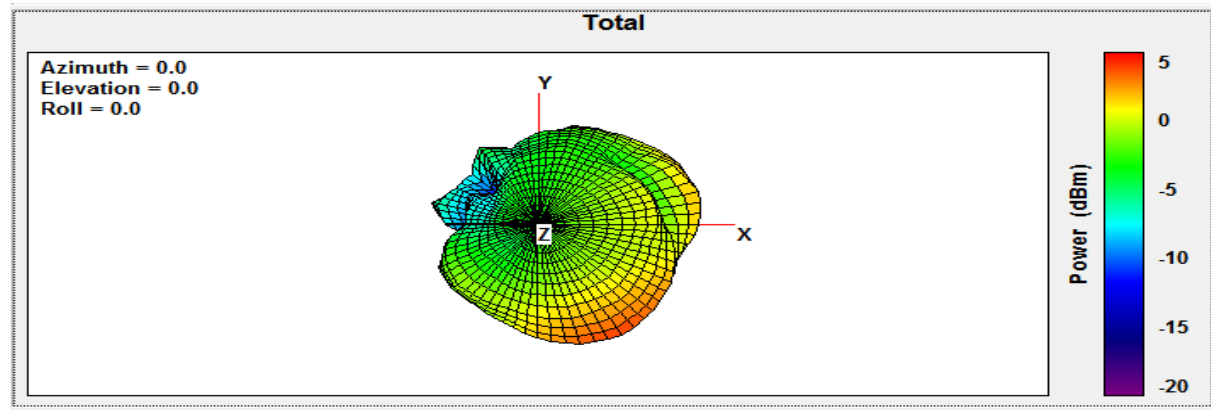
3D Antenna pattern
