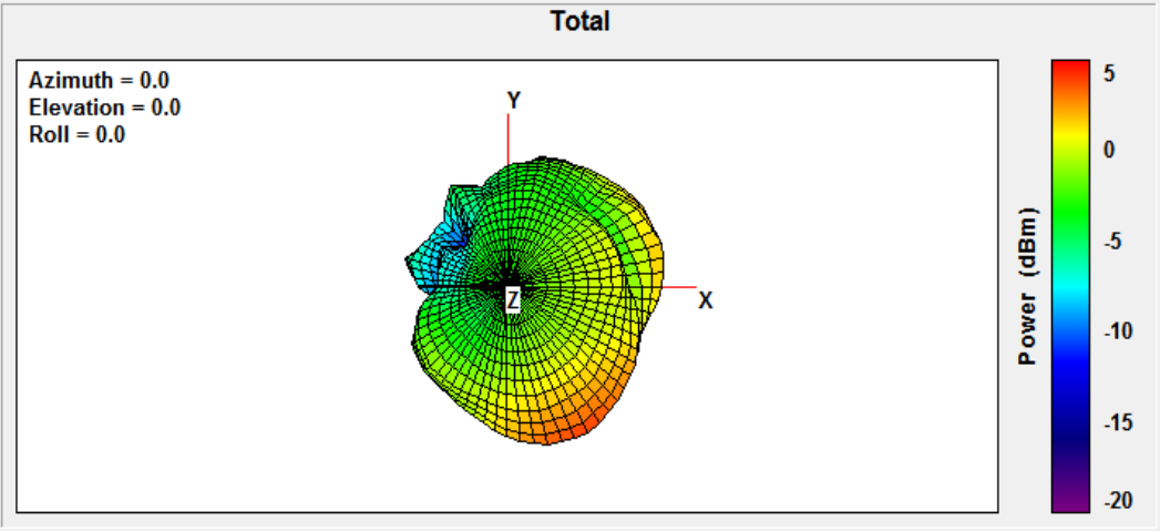
3D Antenna pattern
