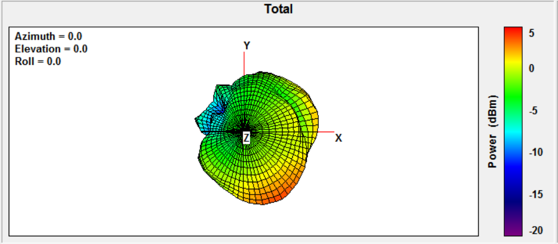
3D Antenna pattern
