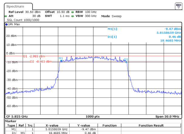
802.11ax20_5825MHz_RU_Full_Chain 1
