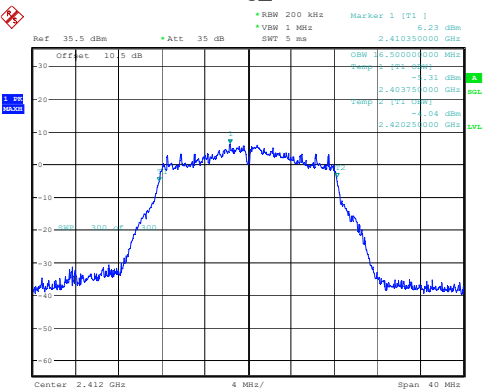
802.11g_2412MHz
