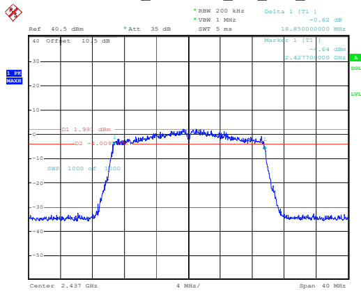
802.11ax20_2437MHz_RU_Full_Chain 0
