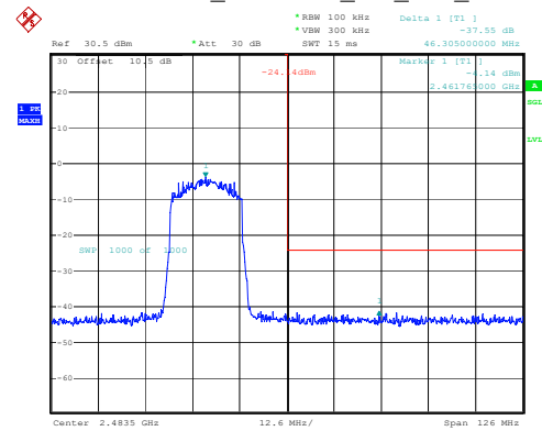
802.11ax20_2462MHz_RU_Full_Chain 1
