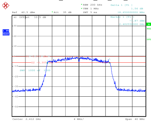
802.11ax20_2412MHz_RU_Full_Chain 1
