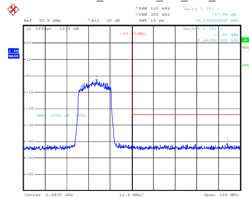
802.11ax20_2462MHz_RU_Full_Chain 0
