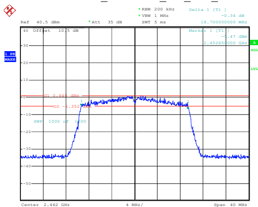
802.11ax20_2462MHz_RU_Full_Chain 1
