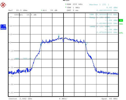
802.11g_2462MHz
