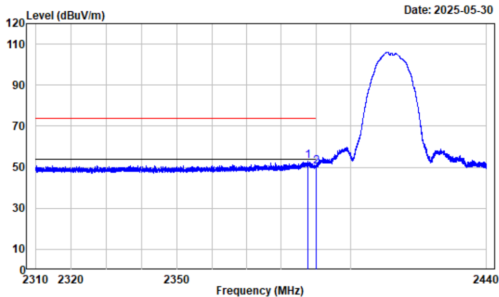
Left Band edge_Horizontal_Peak_802.11b_ANT1
