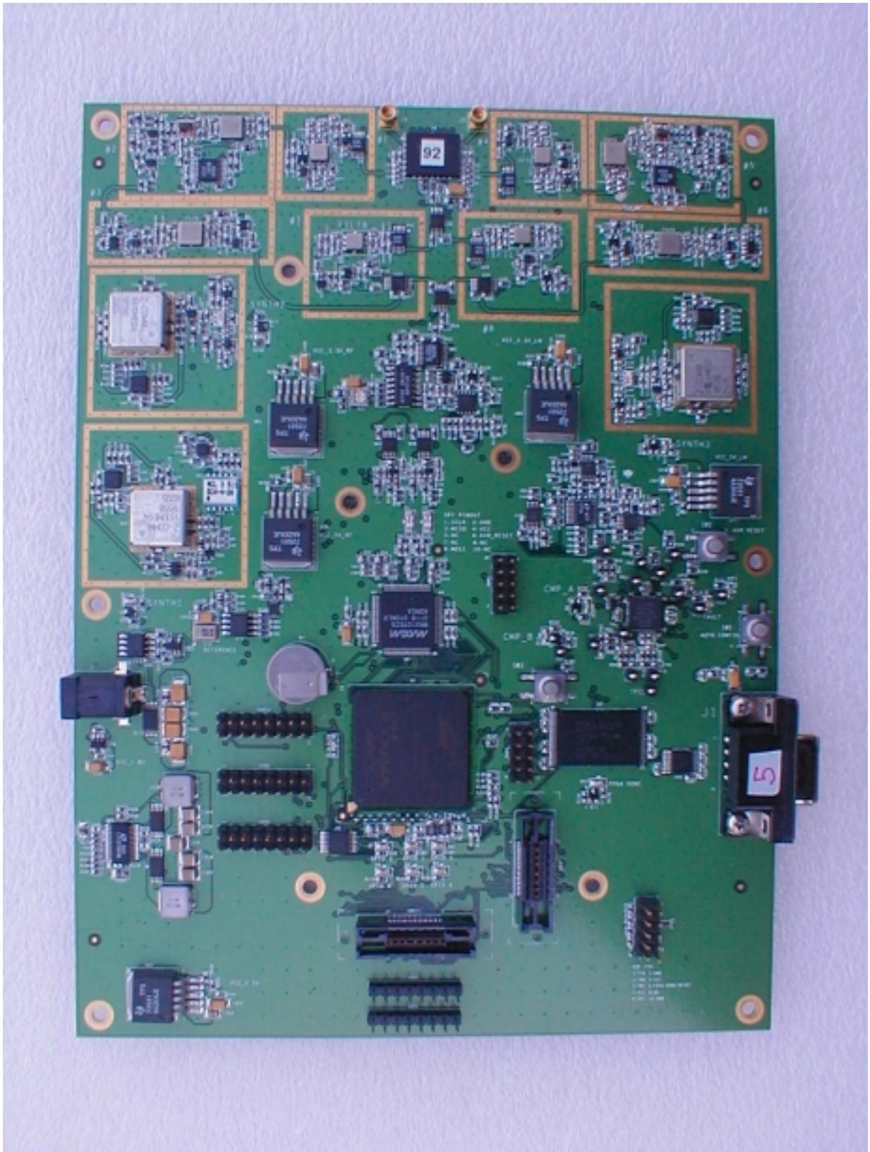
TOP VIEW OF MAIN BOARD (CIRCUIT SHIELDS REMOVED)
