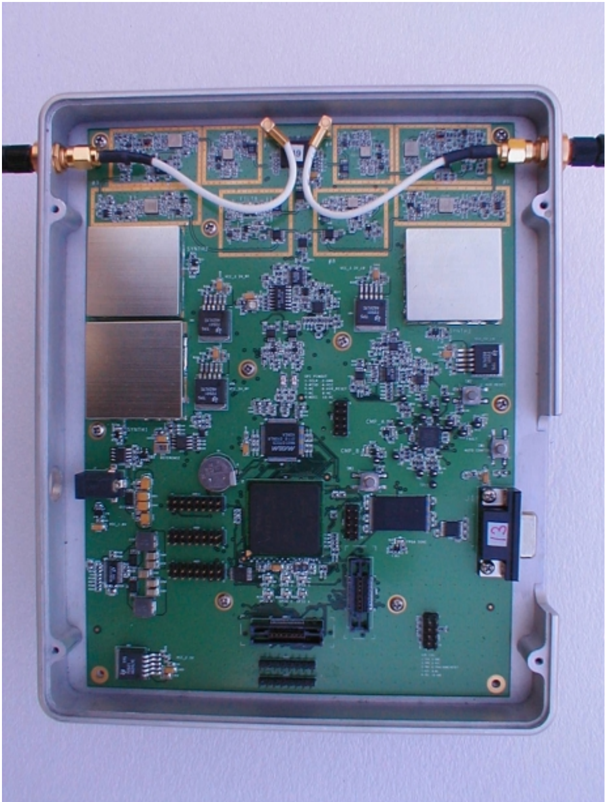
INSIDE VIEW OF EUT
