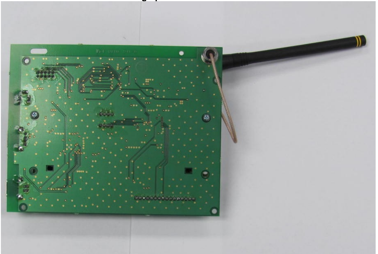
Photograph of PC Board: Foil Side
