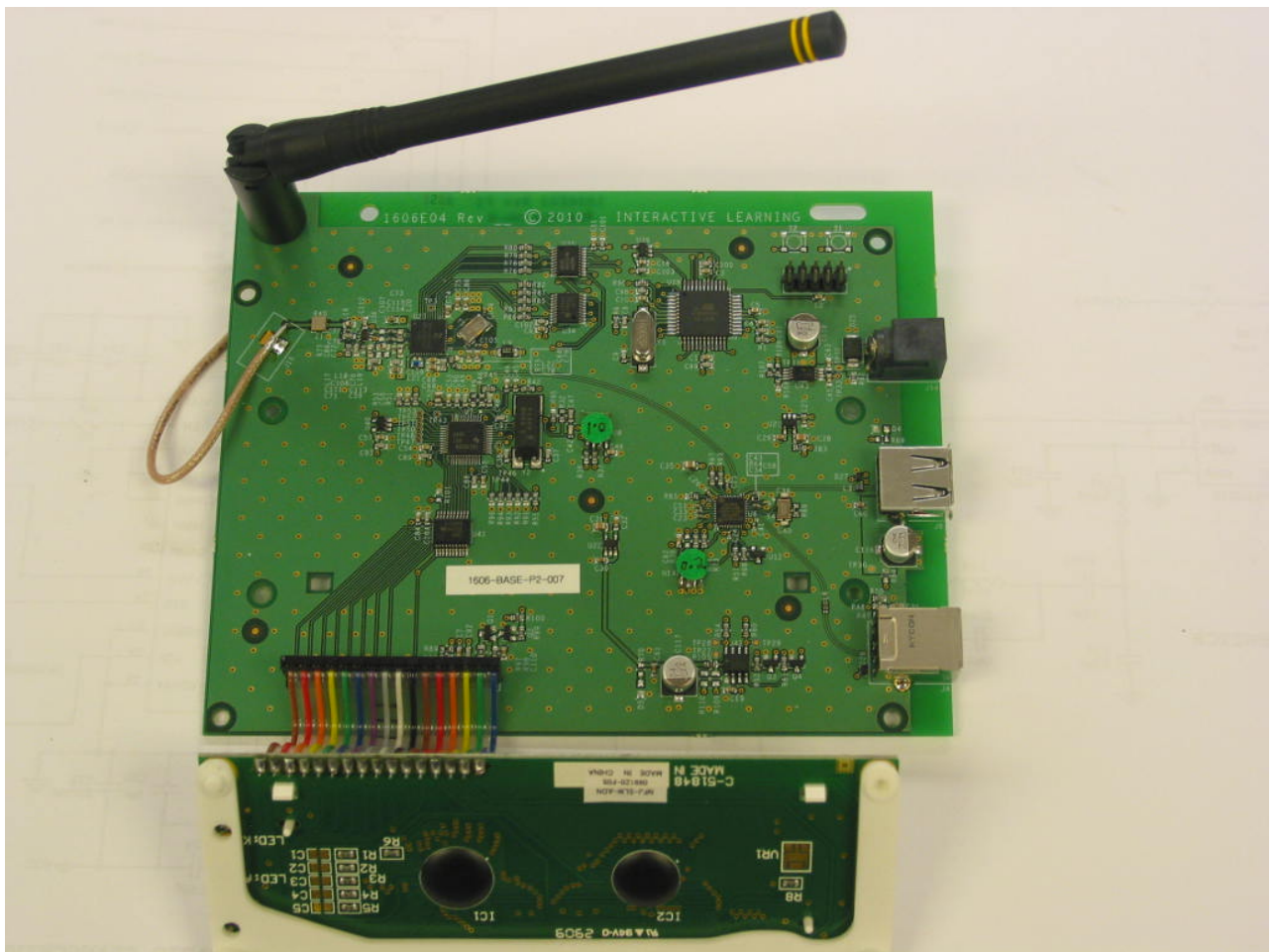
Display board removed; Top Side of PCB
