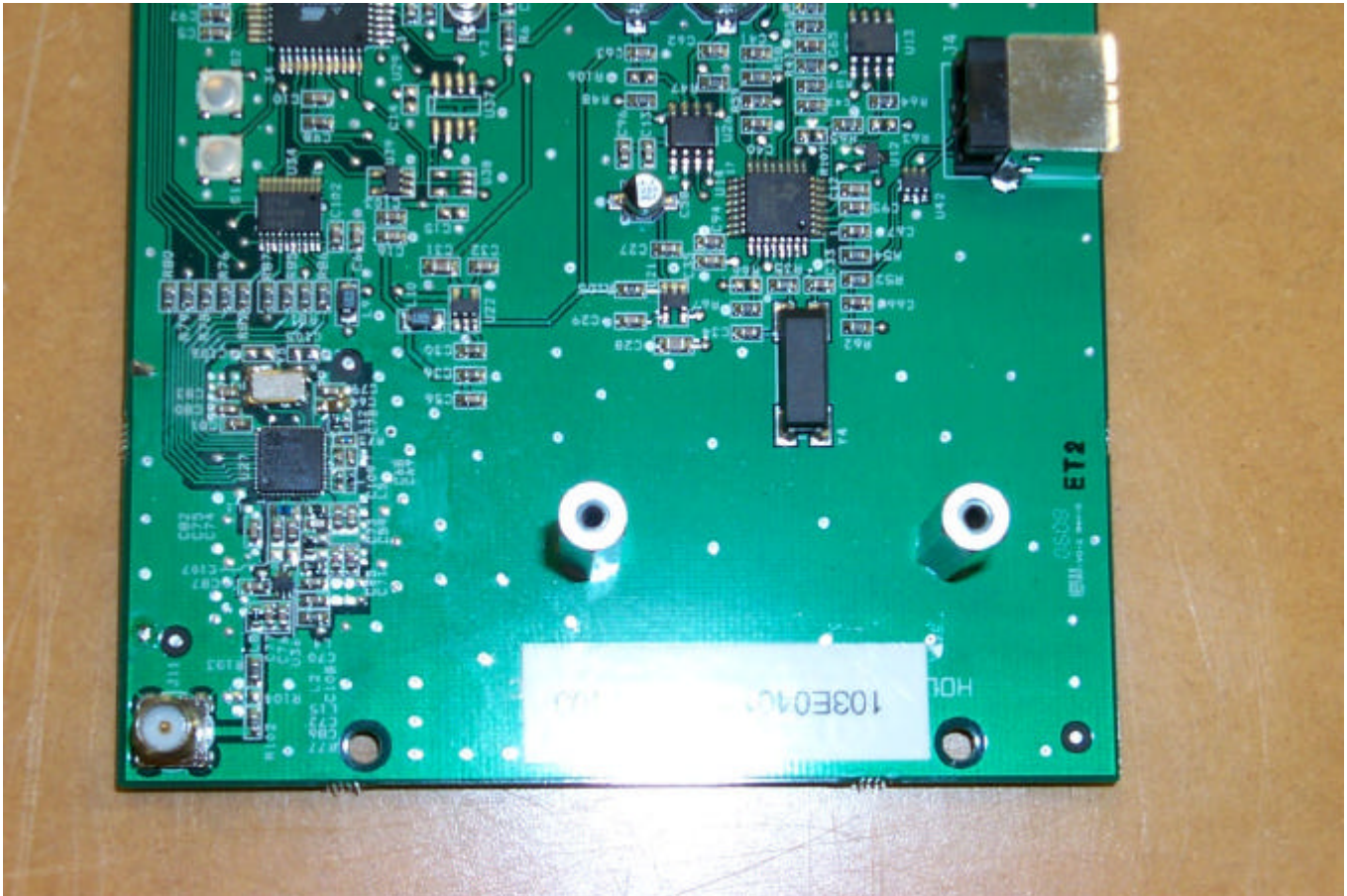
Figure 4 - EUT Internal Photo, Right Side Detail
