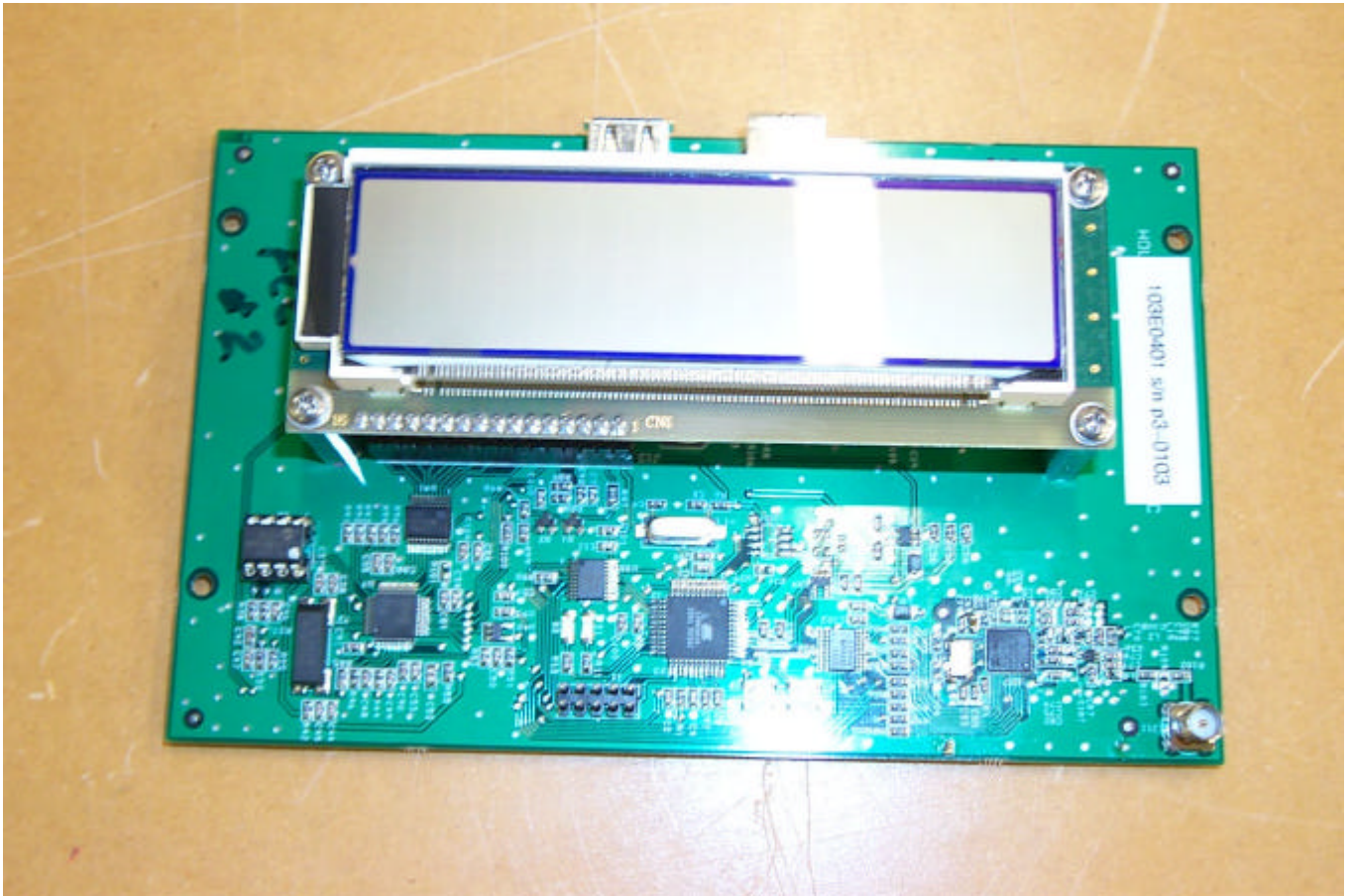
Figure 1 - EUT Internal Photo, with LCD
