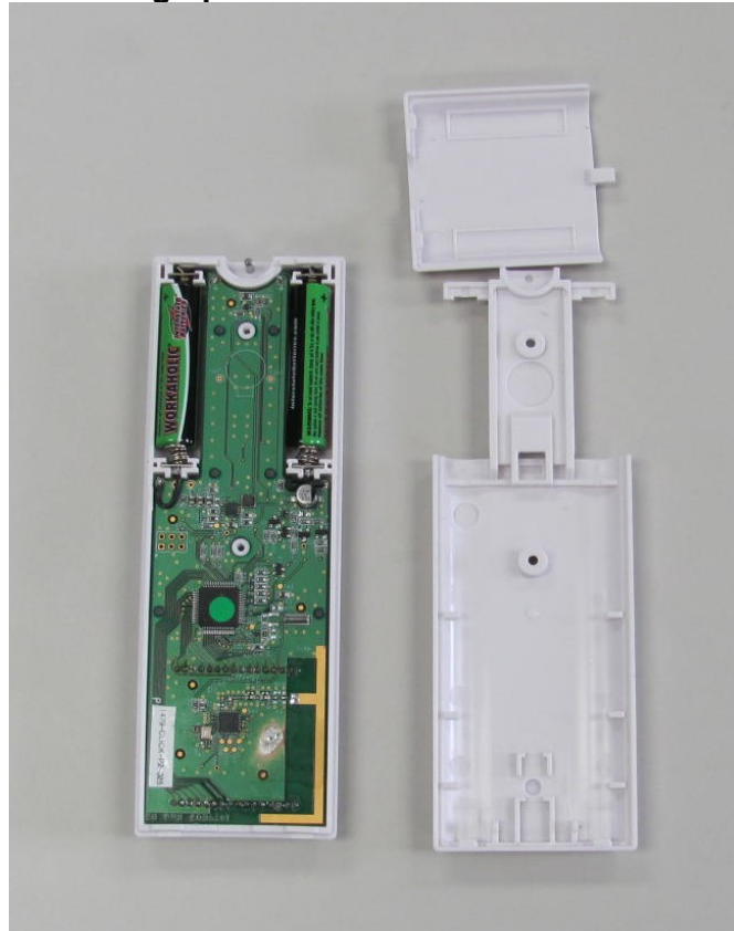
Photograph of EUT: Rear Cover removed
