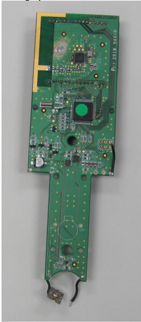
Photograph of PC Board: Foil Side
