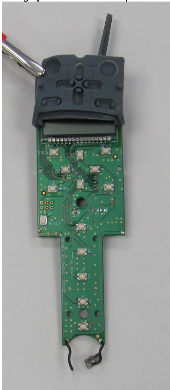
Photograph of PC Board: Component Side
