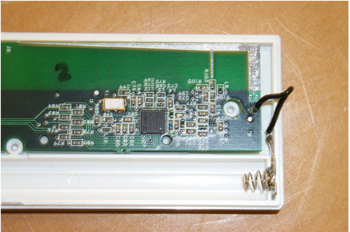
Figure 2 - EUT Internal Photos, Back Side, Bottom Detail
