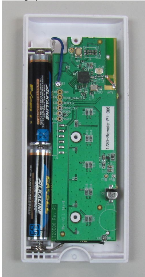
Photograph of EUT: Rear Cover removed
