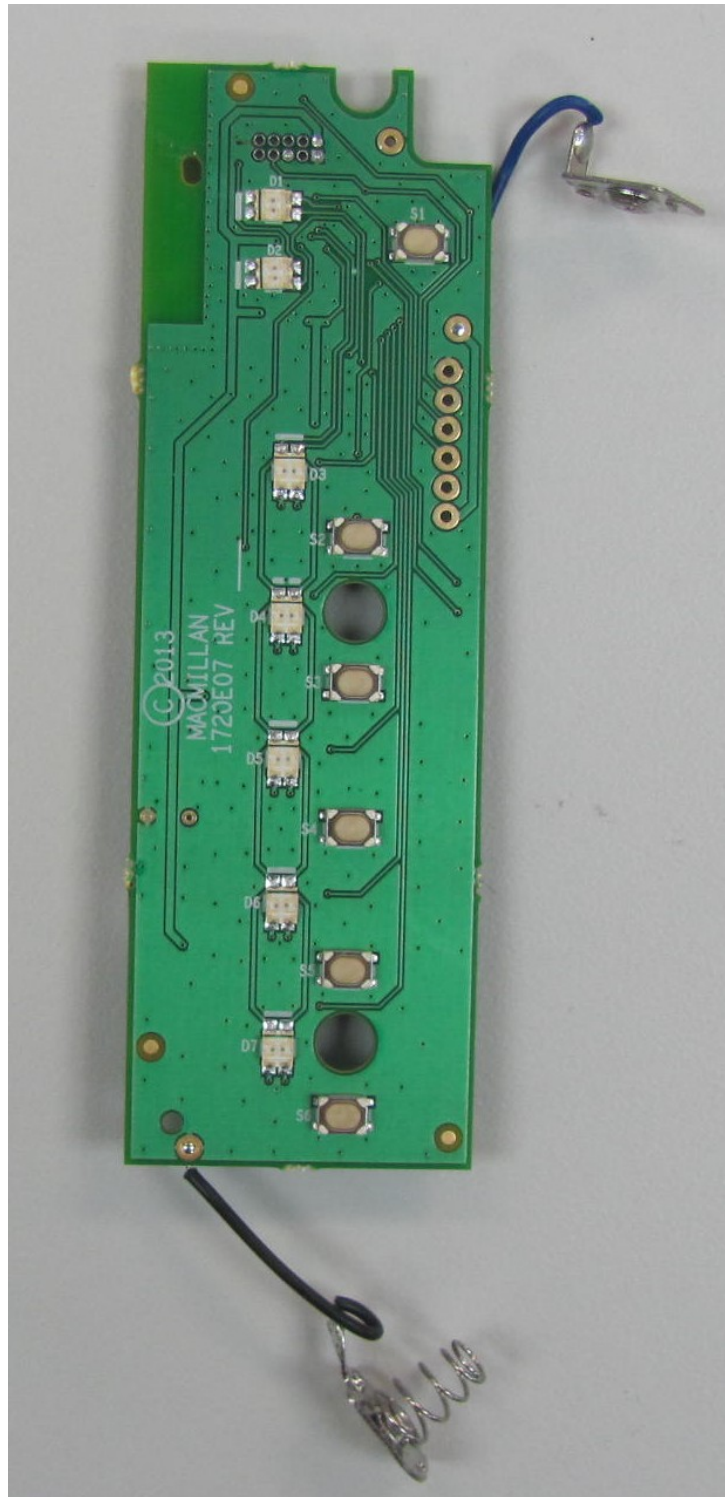
Photograph of PC Board: Foil Side
