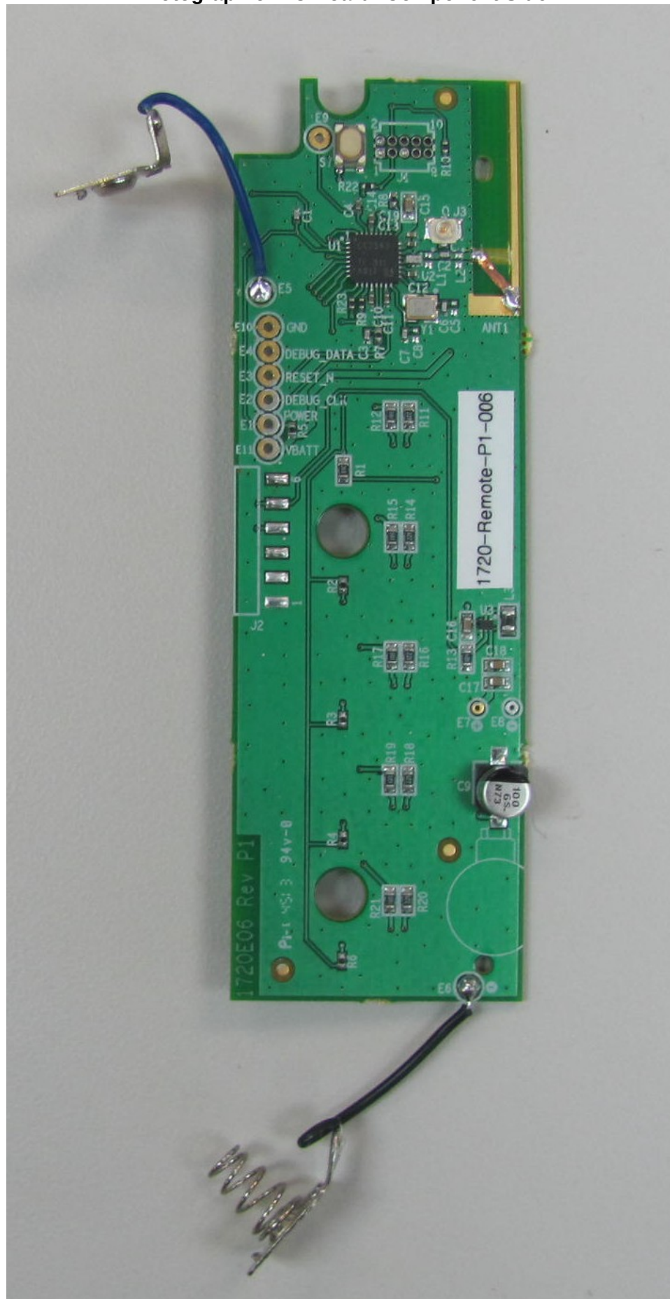
Photograph of PC Board: Component Side
