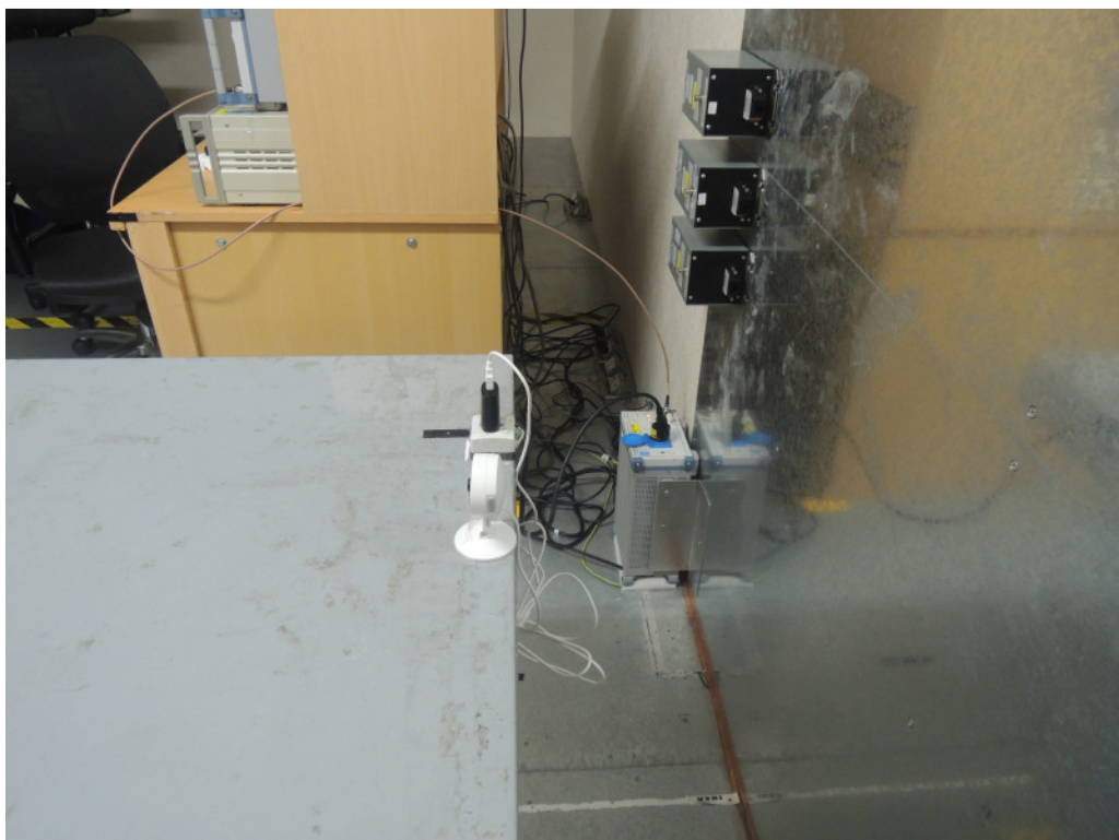
Photograph 6: Set-up for Mains Conducted testing (Back View)
